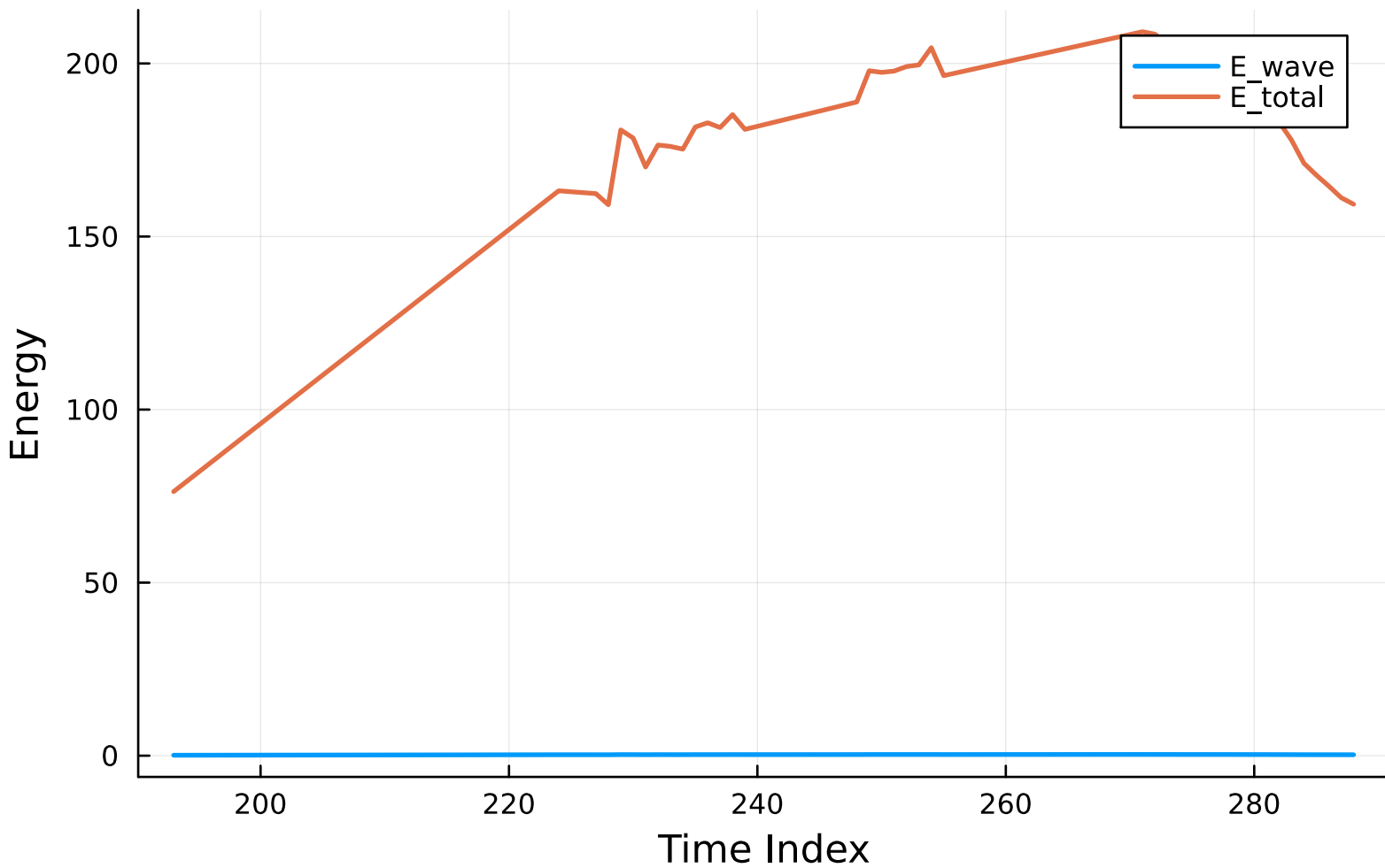
CASES-99 Energy Components (_991004)
