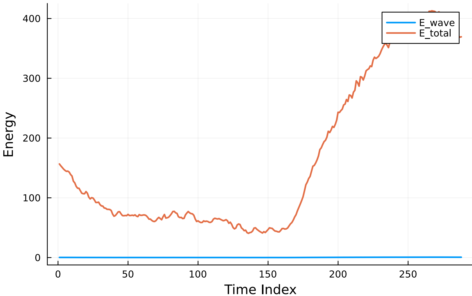
CASES-99 Energy Components (_991005)
