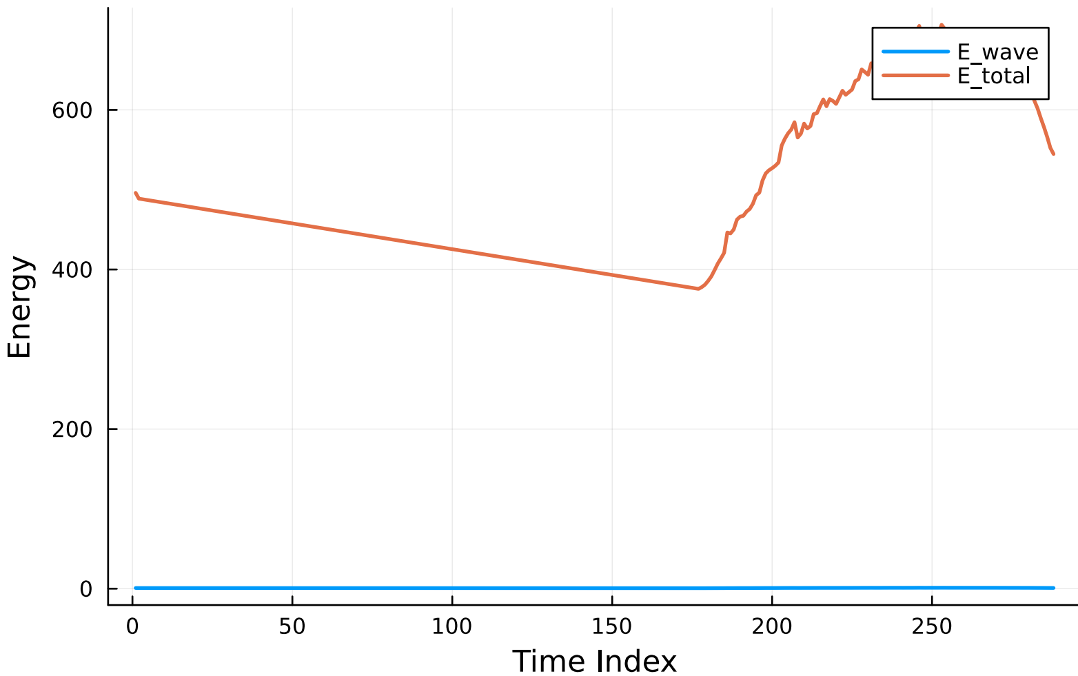
CASES-99 Energy Components (_991012)
