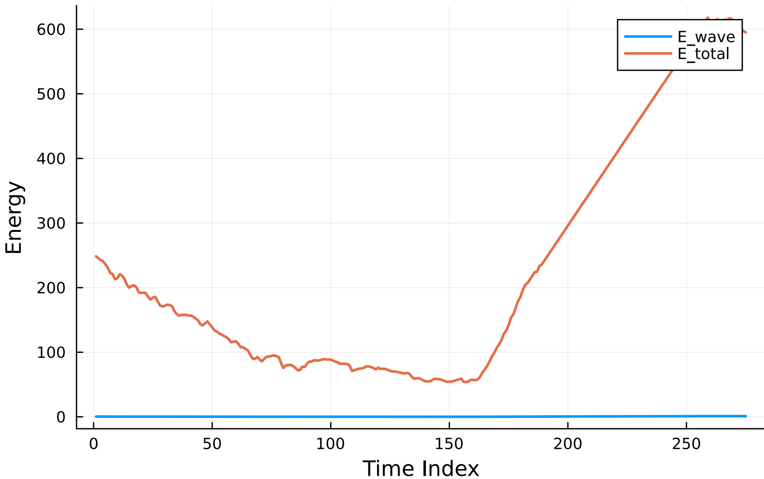
CASES-99 Energy Components (_991014)
