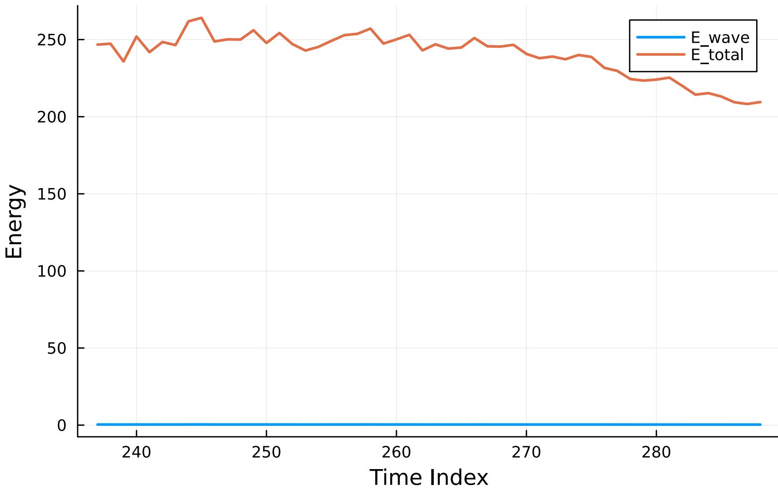
CASES-99 Energy Components (_991016)
