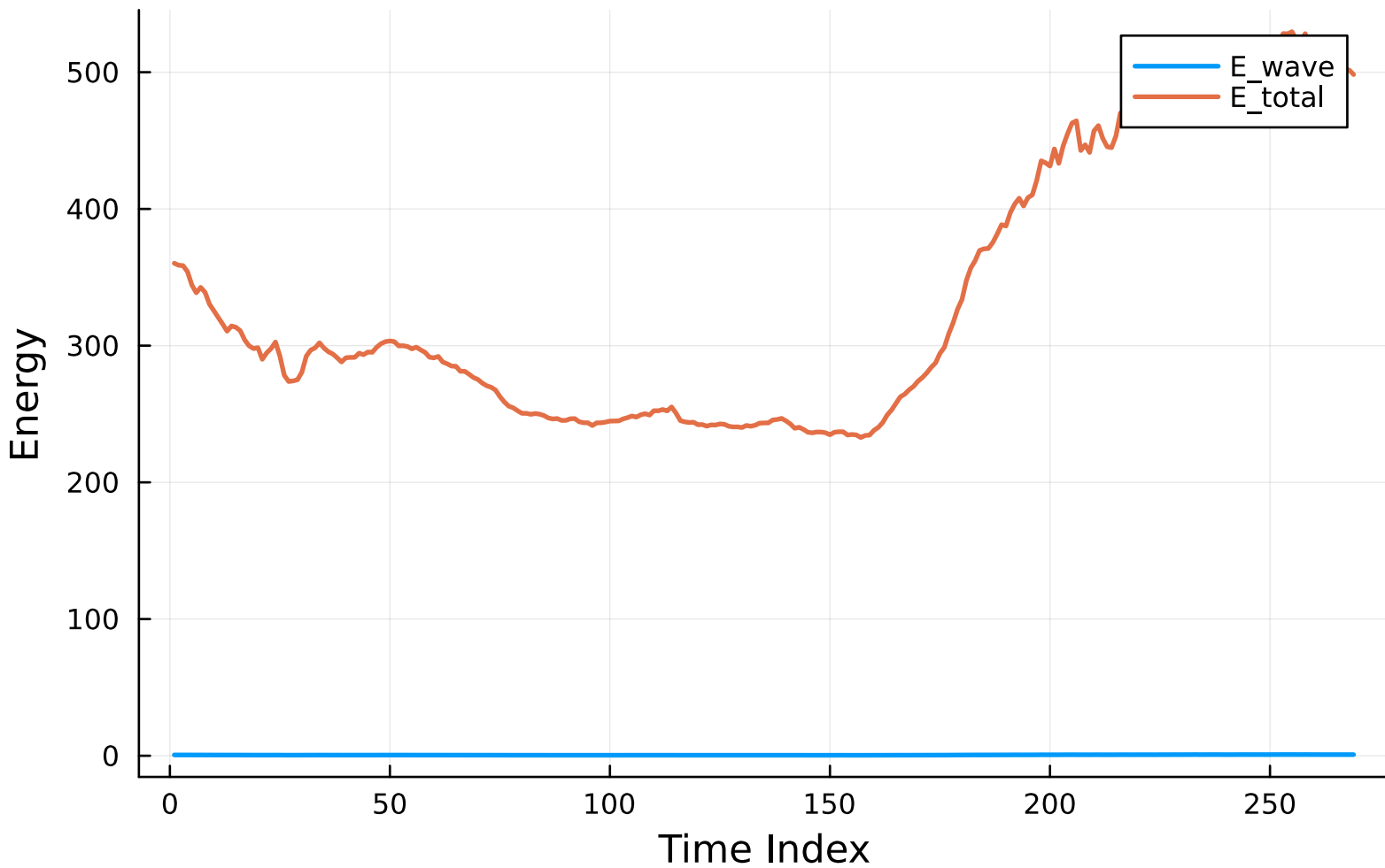
CASES-99 Energy Components (_991029)
