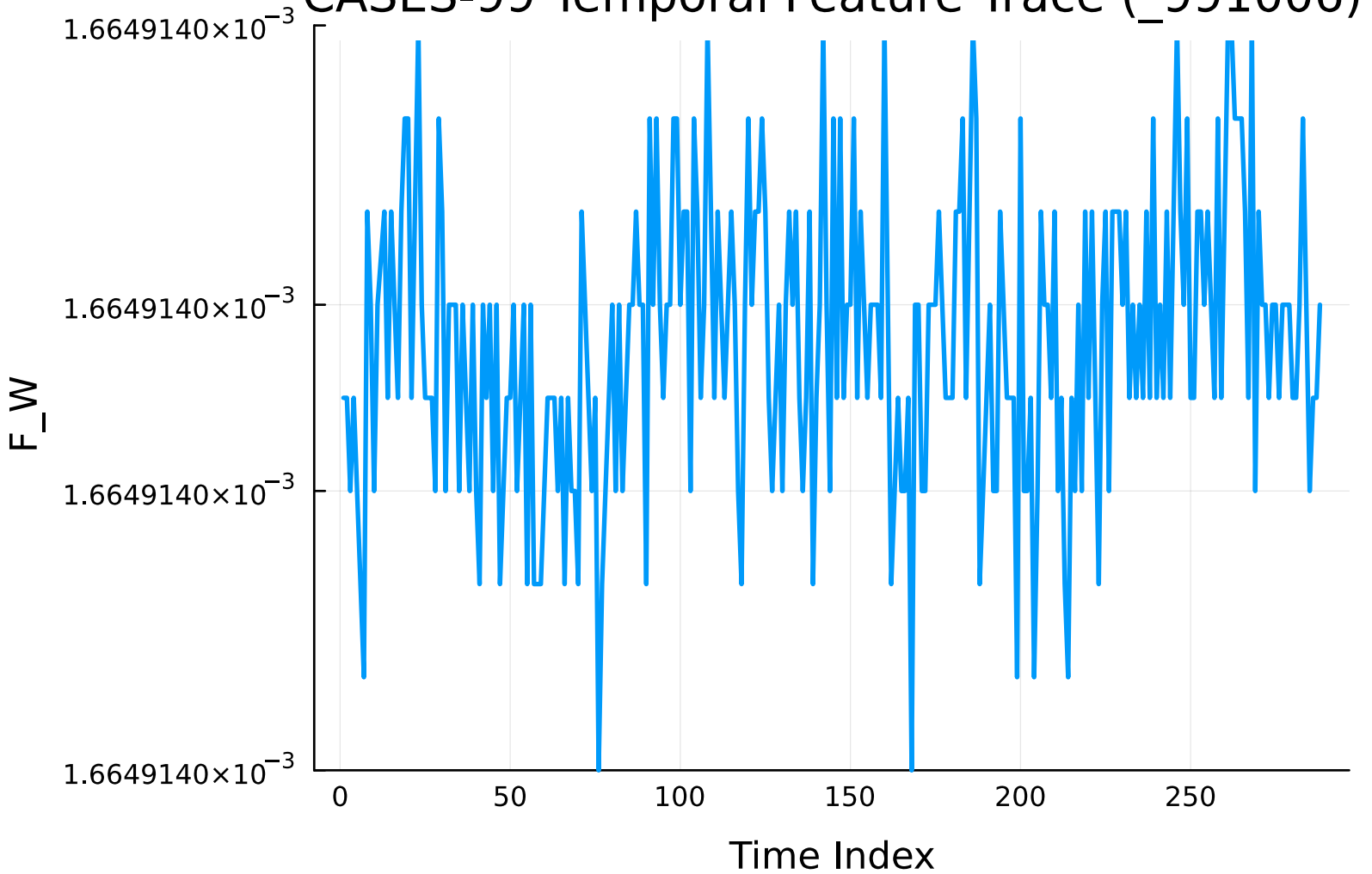
CASES-99 Temporal Feature Trace (_991006)
