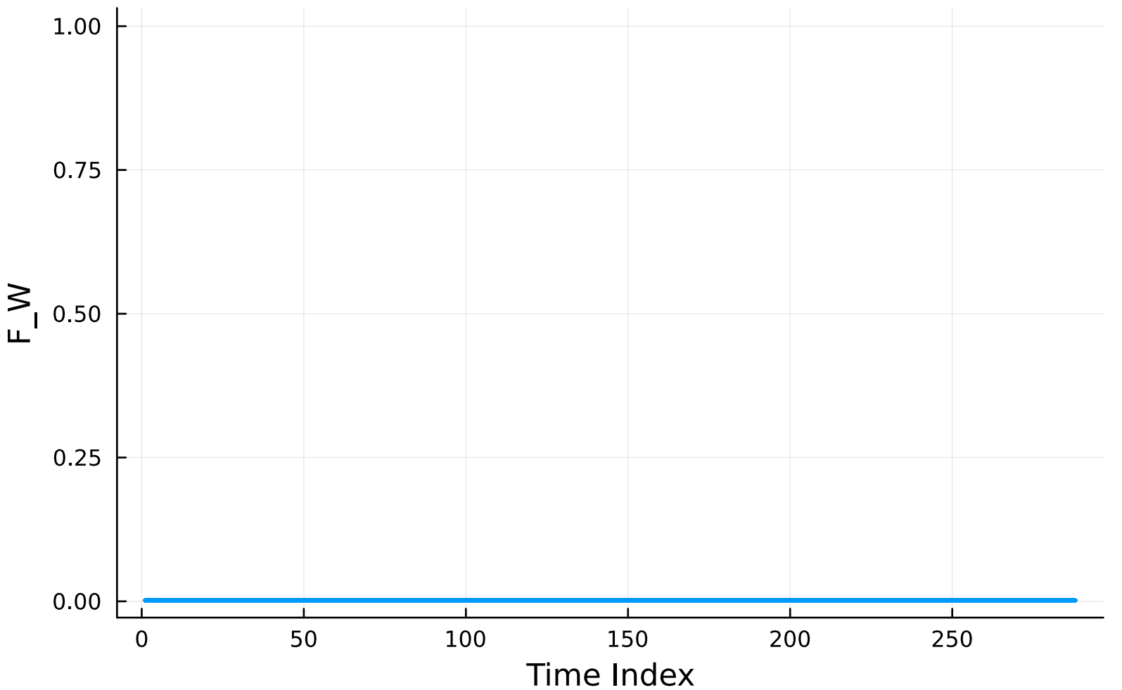
CASES-99 Temporal Feature Trace
