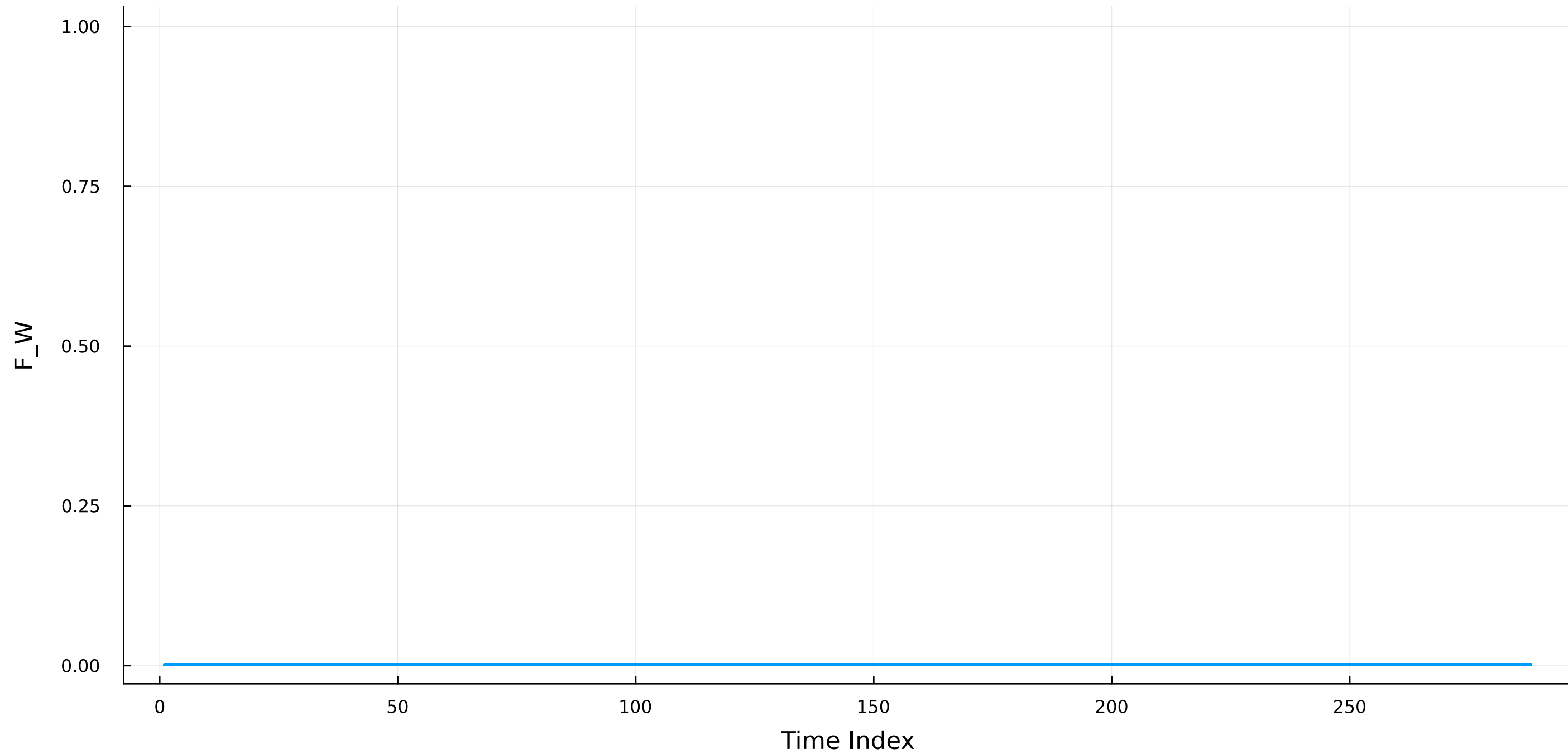
CASES-99 Temporal Feature Trace
