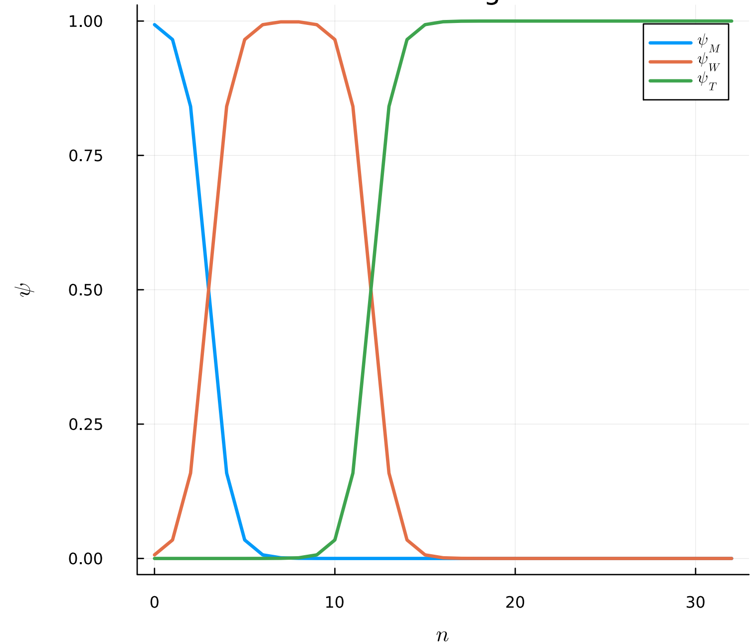
Modal Partitioning Windows
