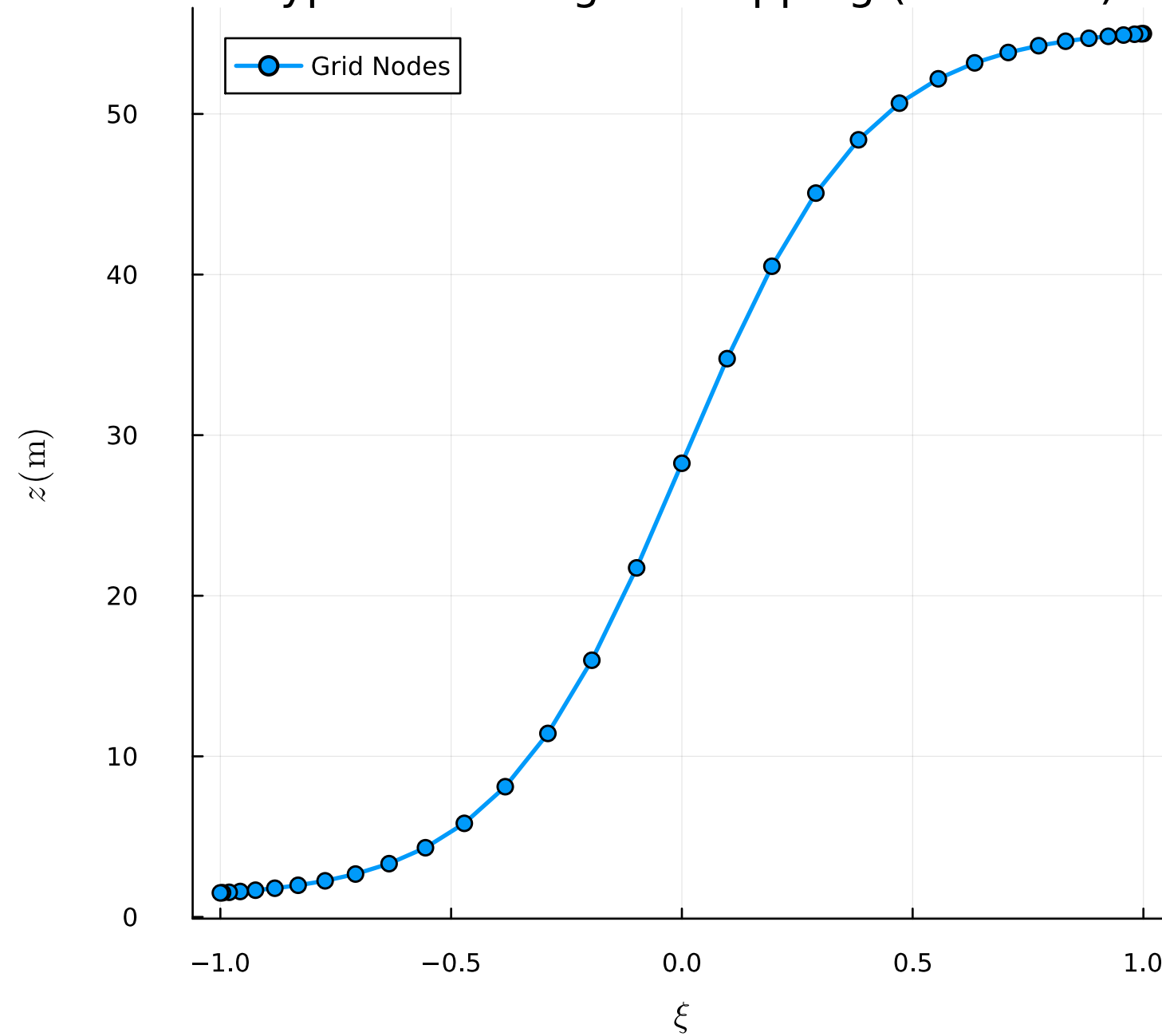
Hyperbolic Tangent Mapping ( \alpha = 2.50 )
