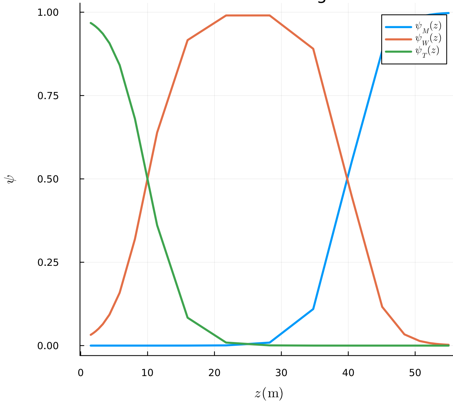
Coordinate Partitioning Windows
