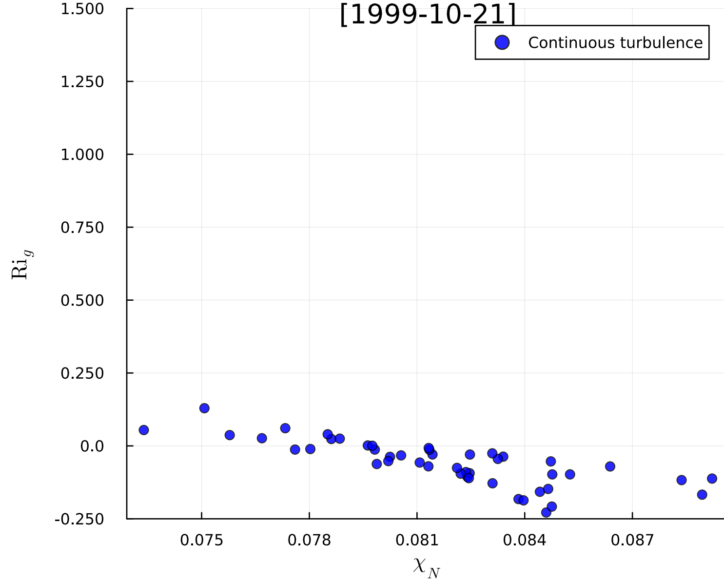
Curvature-Stratification Plane
