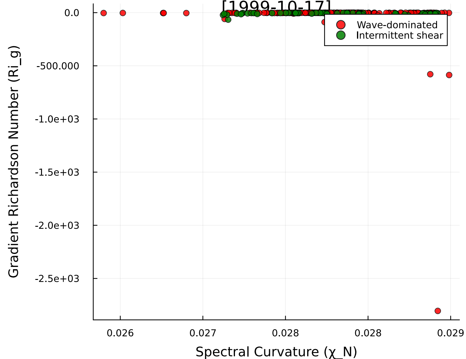
Curvature-Stratification Plane
