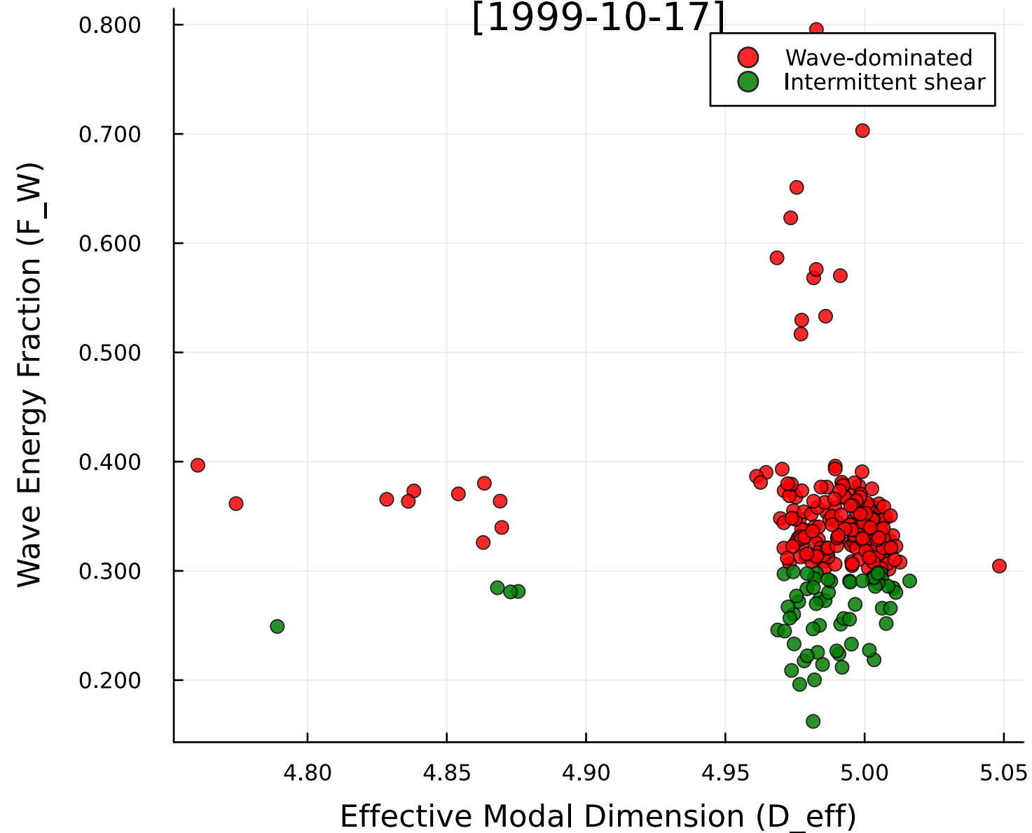
Energy-Dimension Plane
