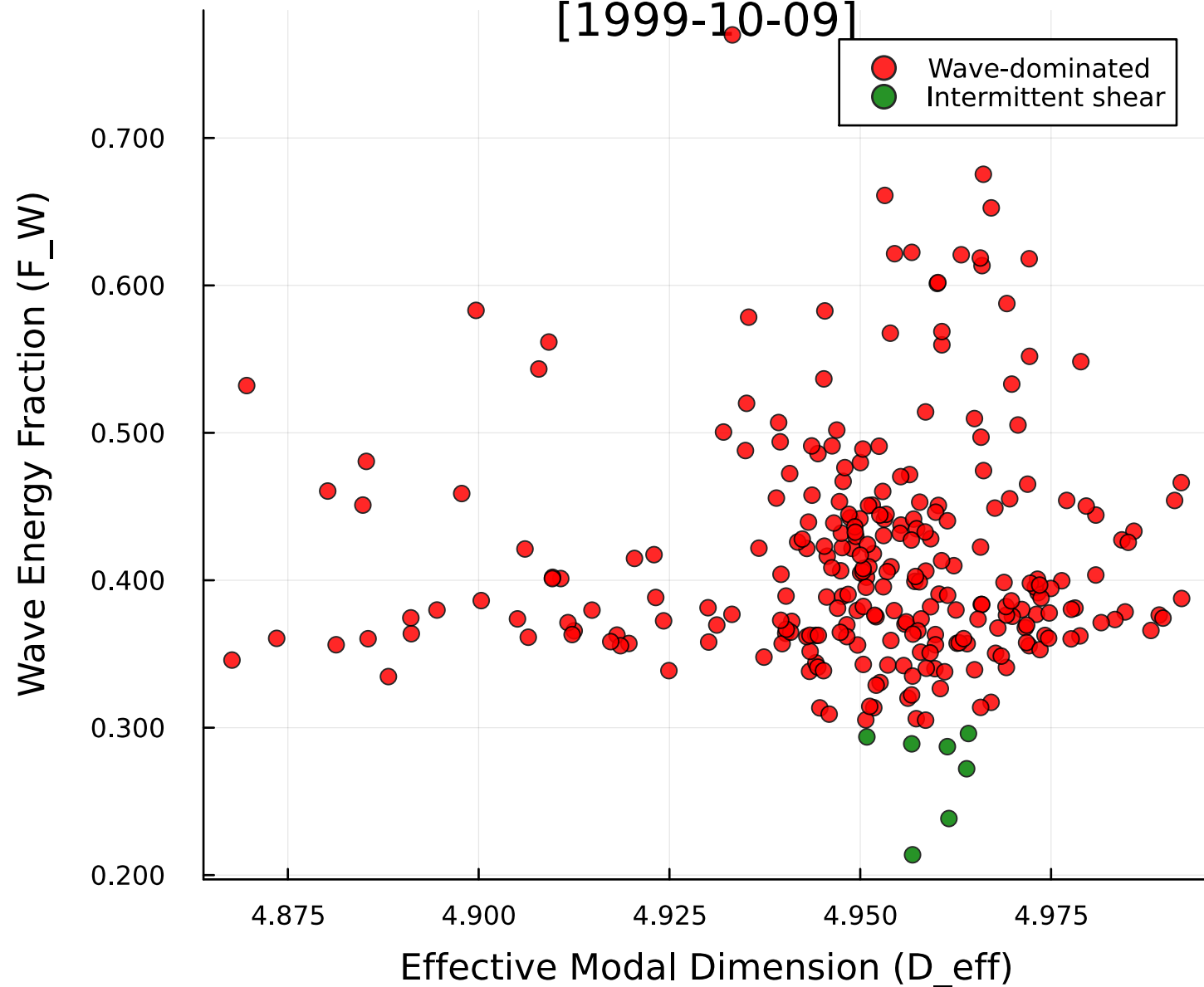
Energy-Dimension Plane
