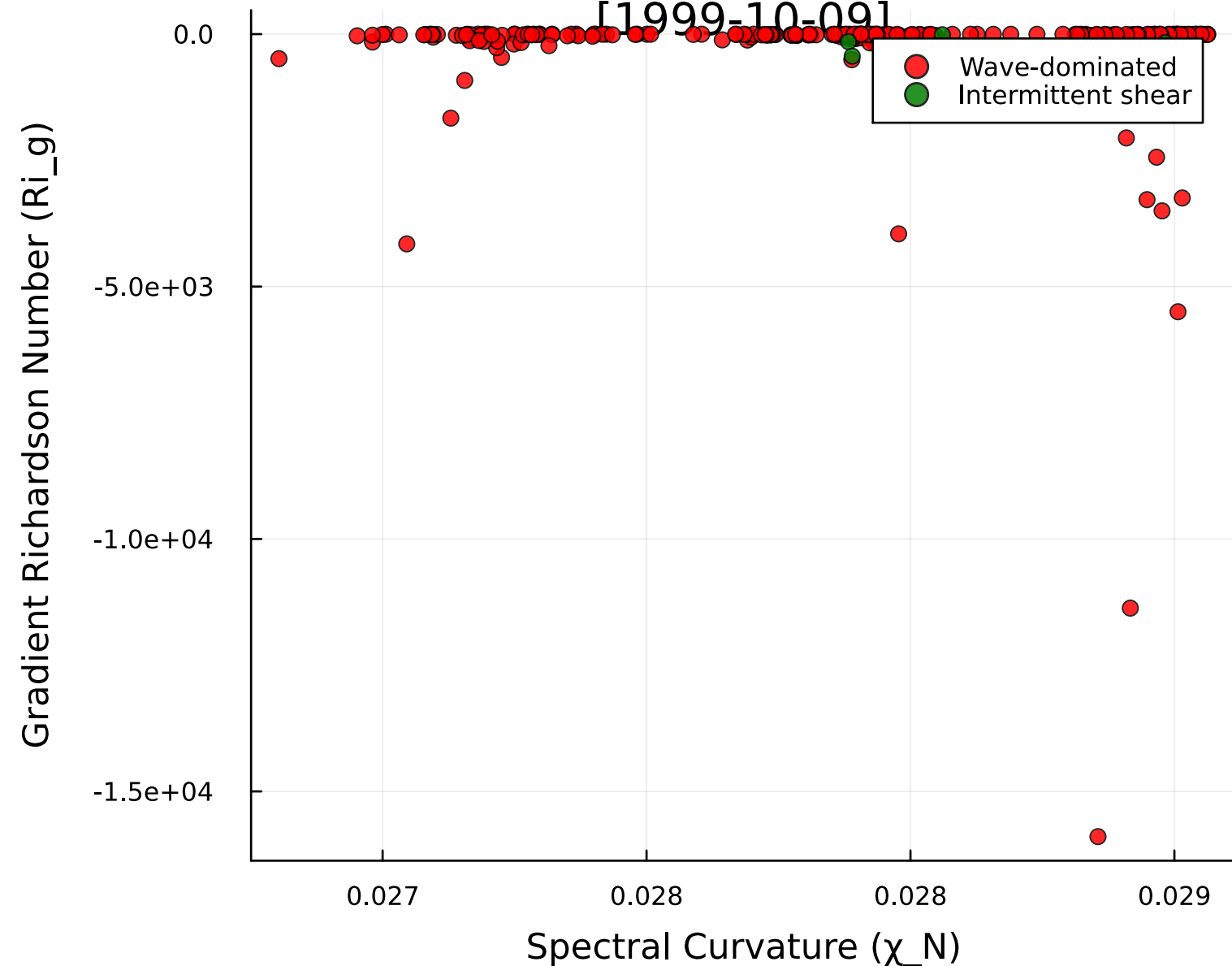
Curvature-Stratification Plane
