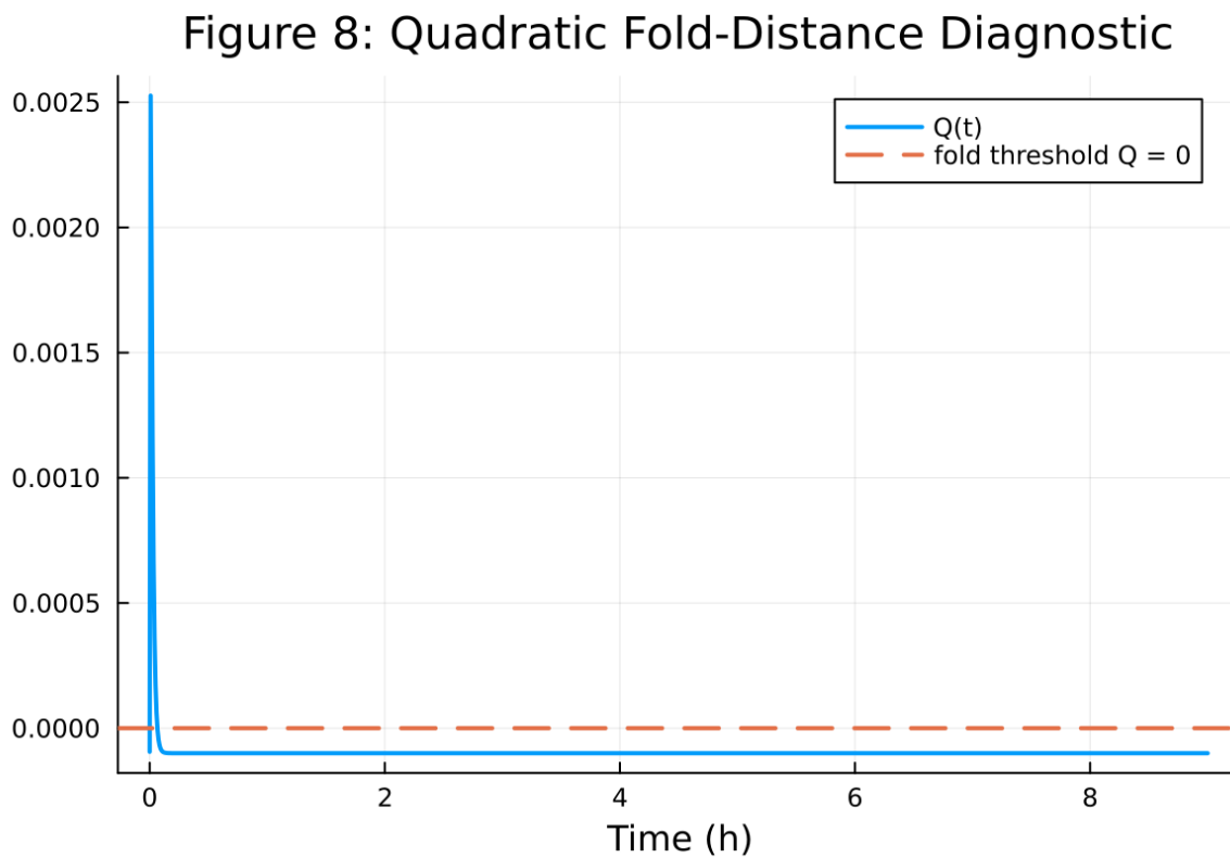
Figure 27: fig08 fold proximity.png
