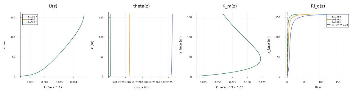
Figure 23: fig04 profiles u theta km.png
