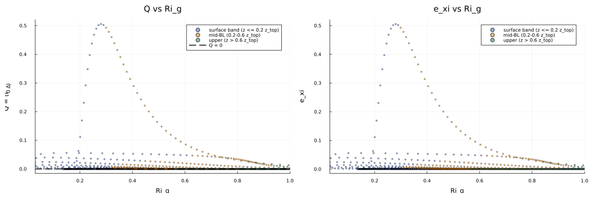
Figure 25: fig06 phase delta exi.png
