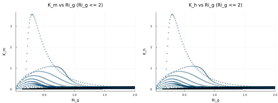
Figure 26: fig07 diffusivity vs ri.png
