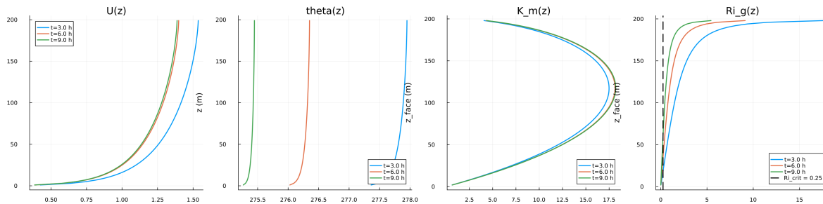
Figure 60: Vertical profiles of U , \theta , and K_m at representative times
