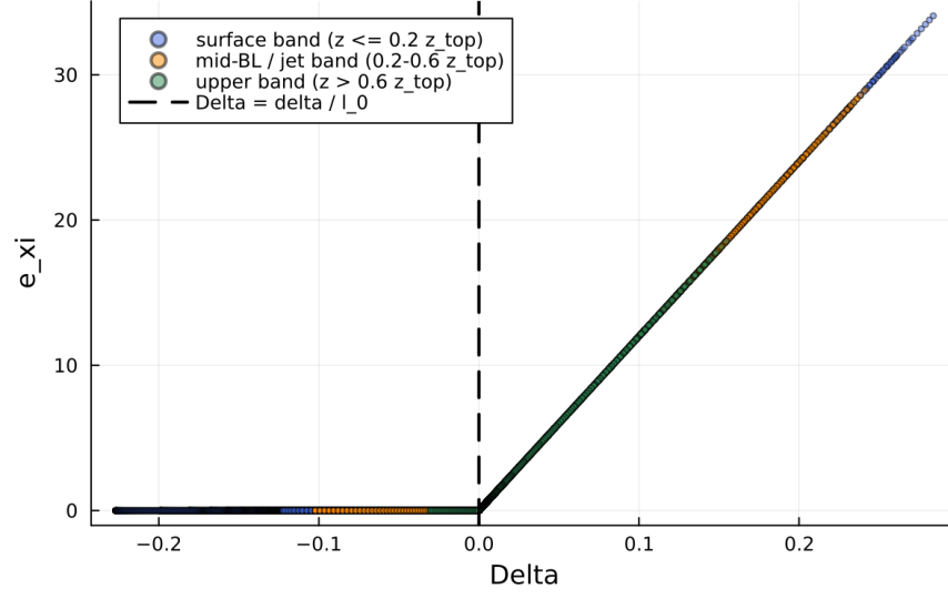
Figure 6: Regularized Slow-Manifold Phase Portrait
