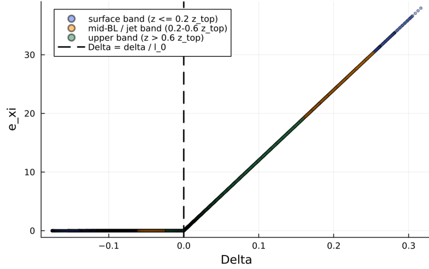
Figure 6: Regularized Slow-Manifold Phase Portrait
