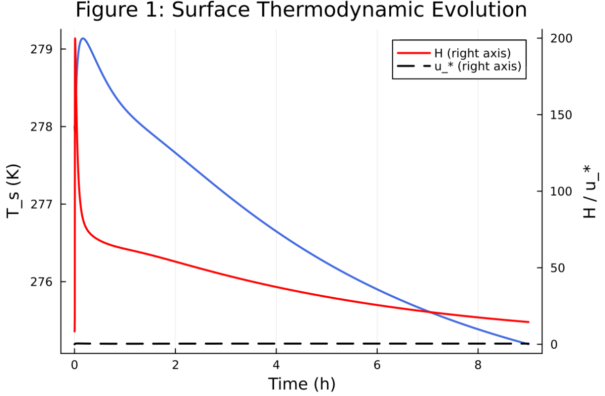
Figure 33: Time series of T_s , sensible heat flux, and friction velocity
