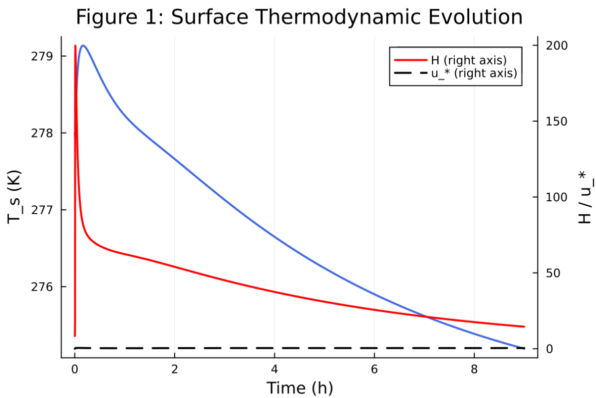
Figure 57: Time series of T_s , sensible heat flux, and friction velocity
