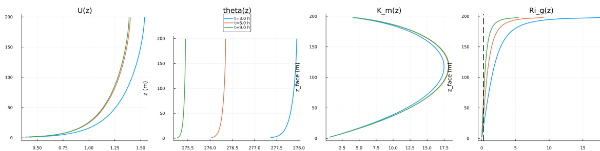
Figure 44: Vertical profiles of U , \theta , and K_m at representative times
