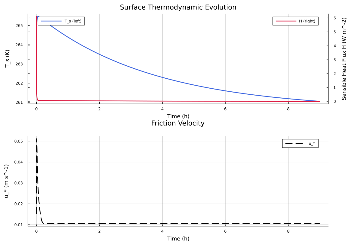
Figure 15: Time series of T_s , sensible heat flux, and friction velocity
