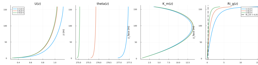
Figure 4: Vertical profiles of U , \theta , and K_m at representative times
