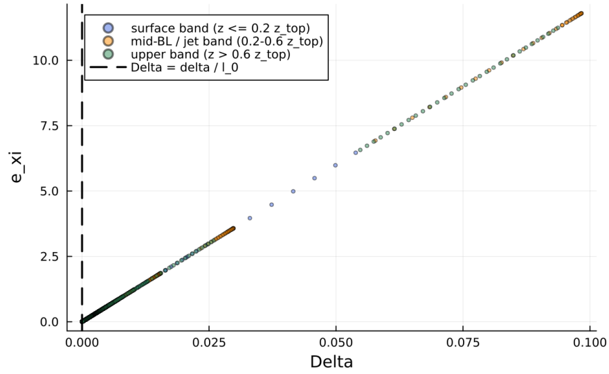
Figure 6: Regularized Slow-Manifold Phase Portrait
