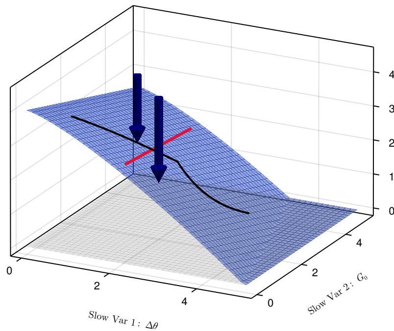
(a) Full Phase Space Geometry ( \mathcal{M}_0 )
