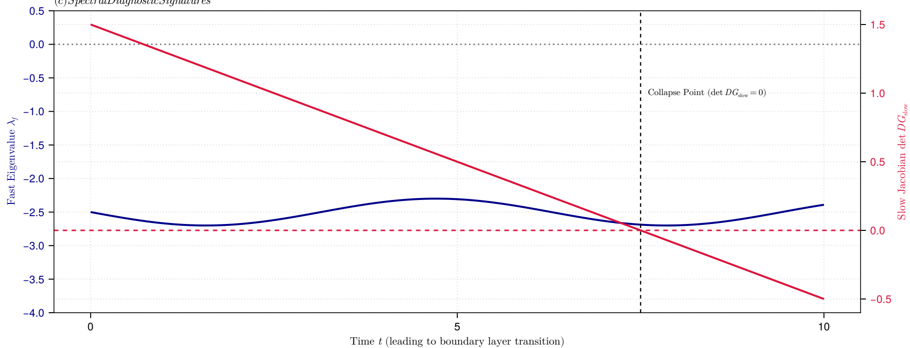
(c) Spectral Diagnostic Signatures
