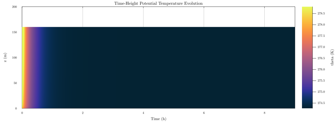
Figure 73: Time-height contour of potential temperature and inversion growth
