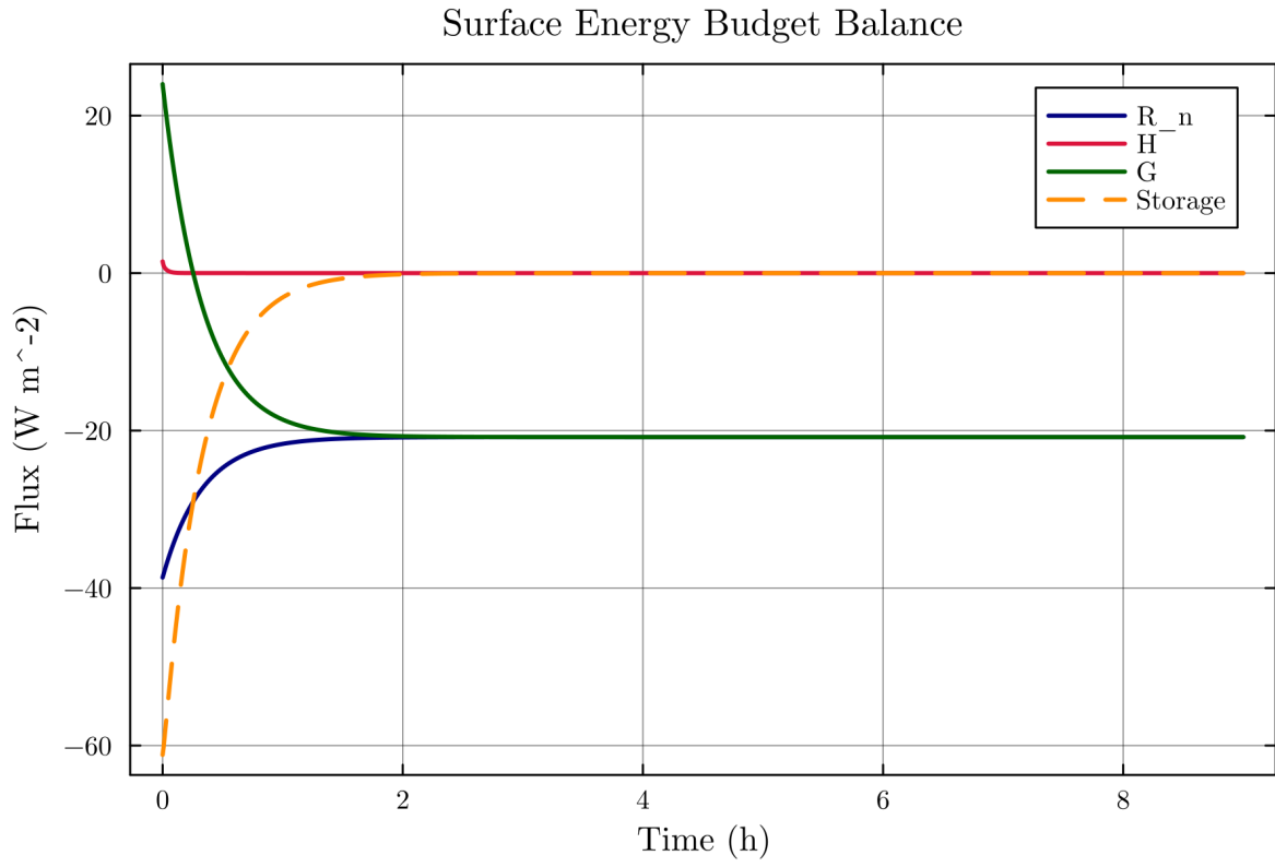
Figure 11: fig05 surface energy budget.png
