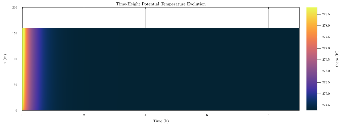
Figure 41: Time-height contour of potential temperature and inversion growth
