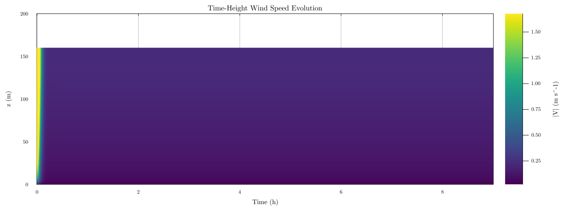
Figure 40: Time-height contour of wind speed with LLJ evolution
