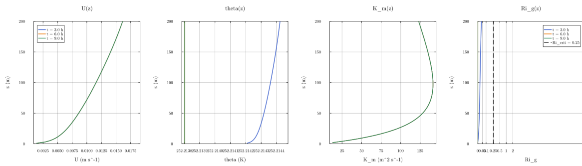
Figure 34: Vertical profiles of U , \theta , and K_m at representative times
