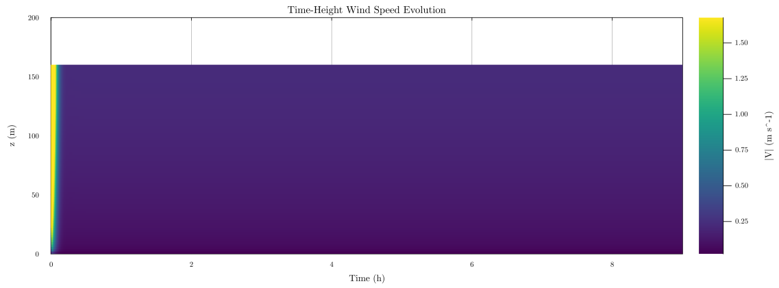
Figure 72: Time-height contour of wind speed with LLJ evolution
