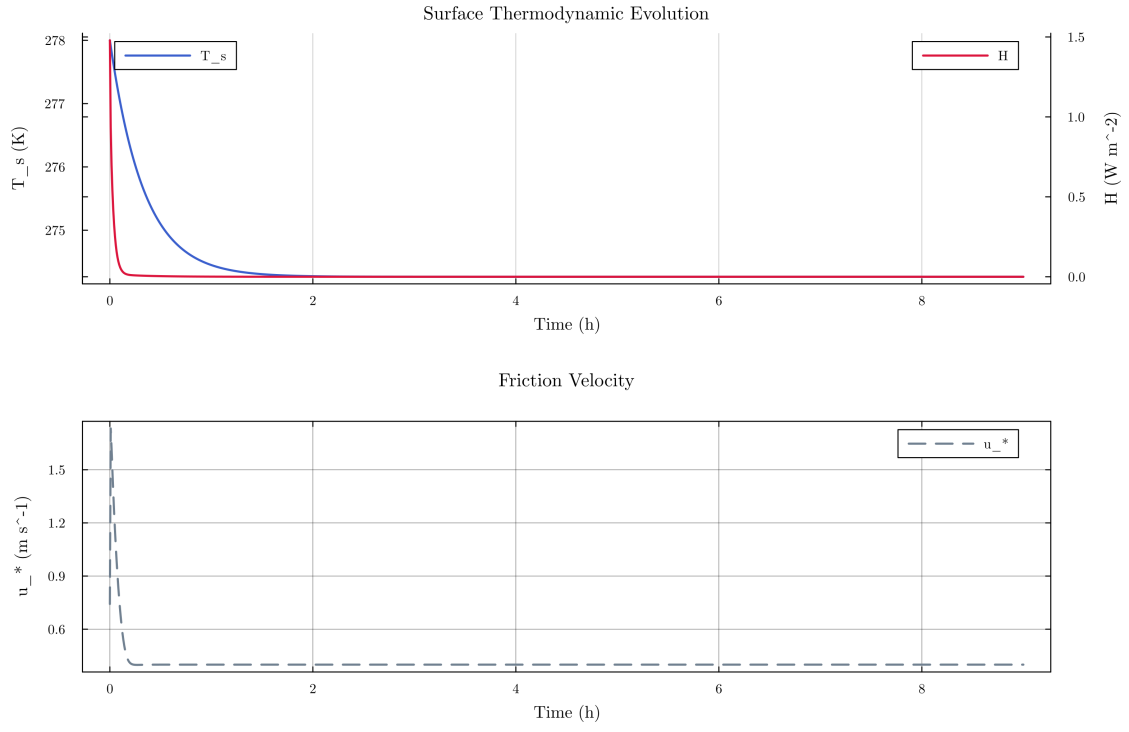
Figure 16: Time series of T_s , sensible heat flux, and friction velocity
