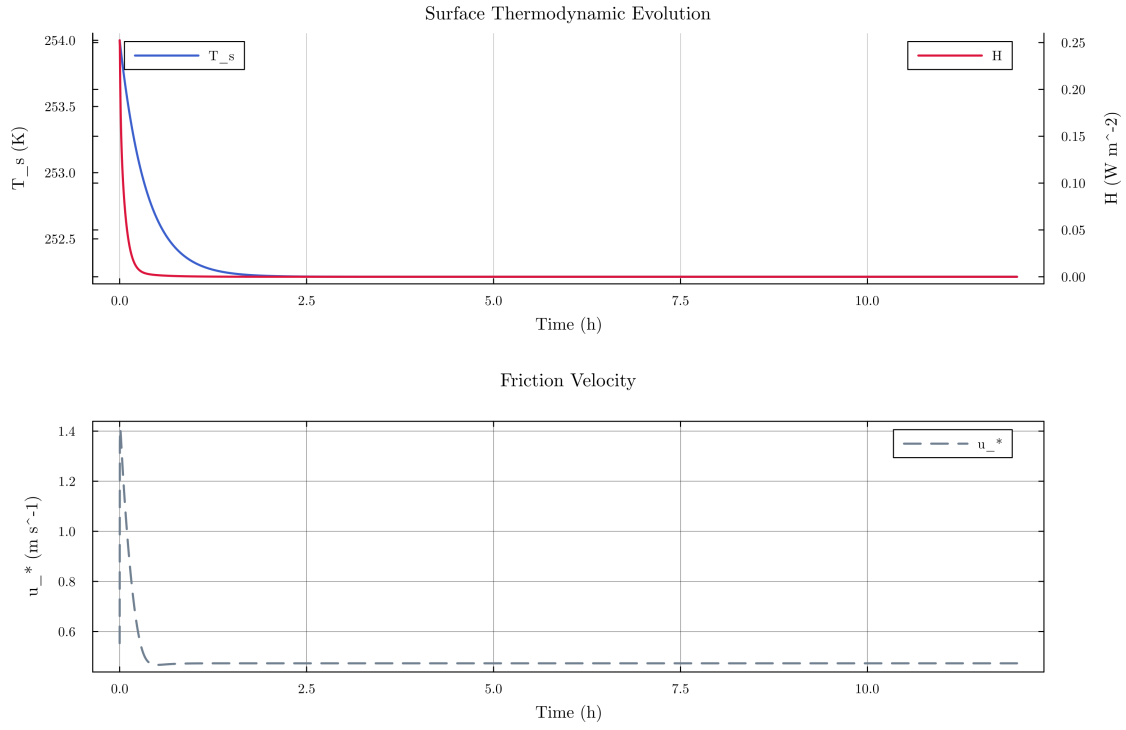
Figure 31: Time series of T_s , sensible heat flux, and friction velocity
