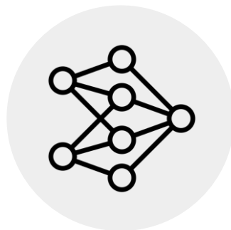
CNN Debugging
