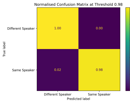
Figure 6: Normalised confusion matrix at threshold 0.98.
