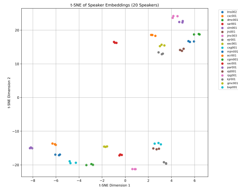
Figure 8: t-SNE visualisation of speaker embeddings for around 20 selected speakers.
