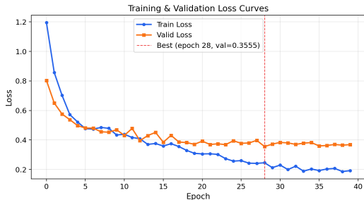
Figure: Train/Validation Loss Curves
