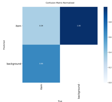
Figure: Normalized Confusion Matrix
