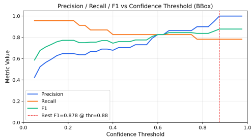
Figure: Score Threshold vs. P/R/F1 (IoU \geq 0.5)
