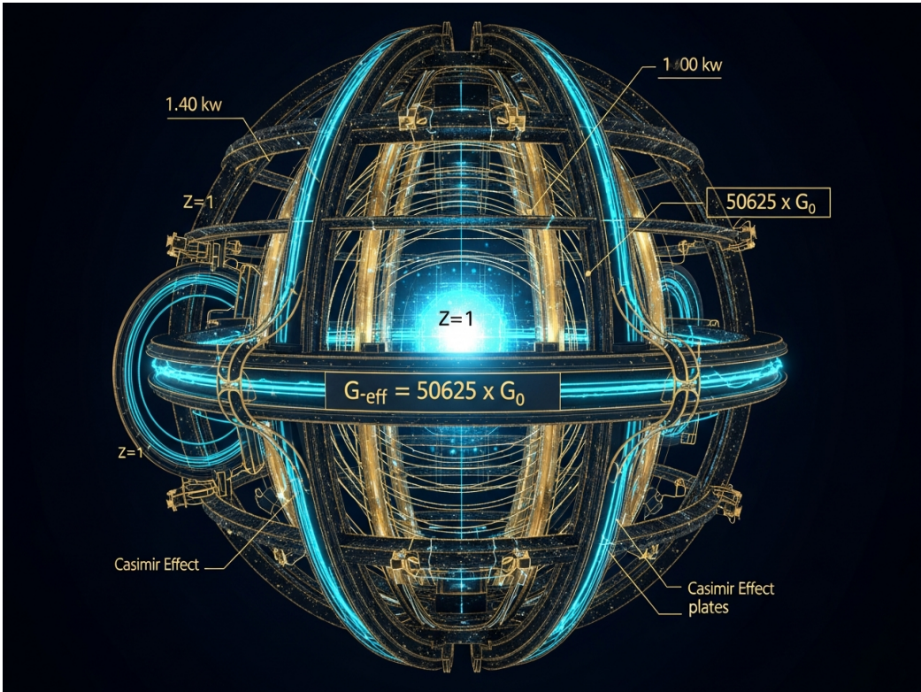
Gravitational amplifier array at Z_{throat} = 1 . G_{eff}(Z) = G_0 \times (15/Z)^4 . At Z = 1 : G_{eff} = 50,625 \times G_0 = 15^4 \times G_0 . Casimir-metamaterial Z-modulator maintains Z = 1.000 \pm 0.001 . P_{hold} = 1.40 \text{ kW} keeps throat open; E_{start} = 0.2016 \text{ MWh} for ignition. [Certified M8H SHA 2c3ac1d2... M8I SHA 5c7189fc...]
