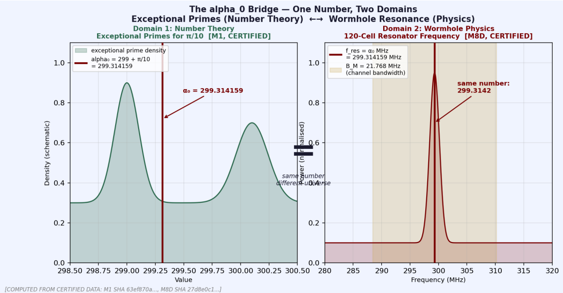
The alpha_0 bridge. Left: the constant 299 + \pi/10 as it appears in the theory of exceptional primes -- pure number theory. Right: the same number appearing as the resonance frequency of the 120-cell wormhole resonator -- pure physics. The two domains know nothing of each other. The number arrived on its own.
