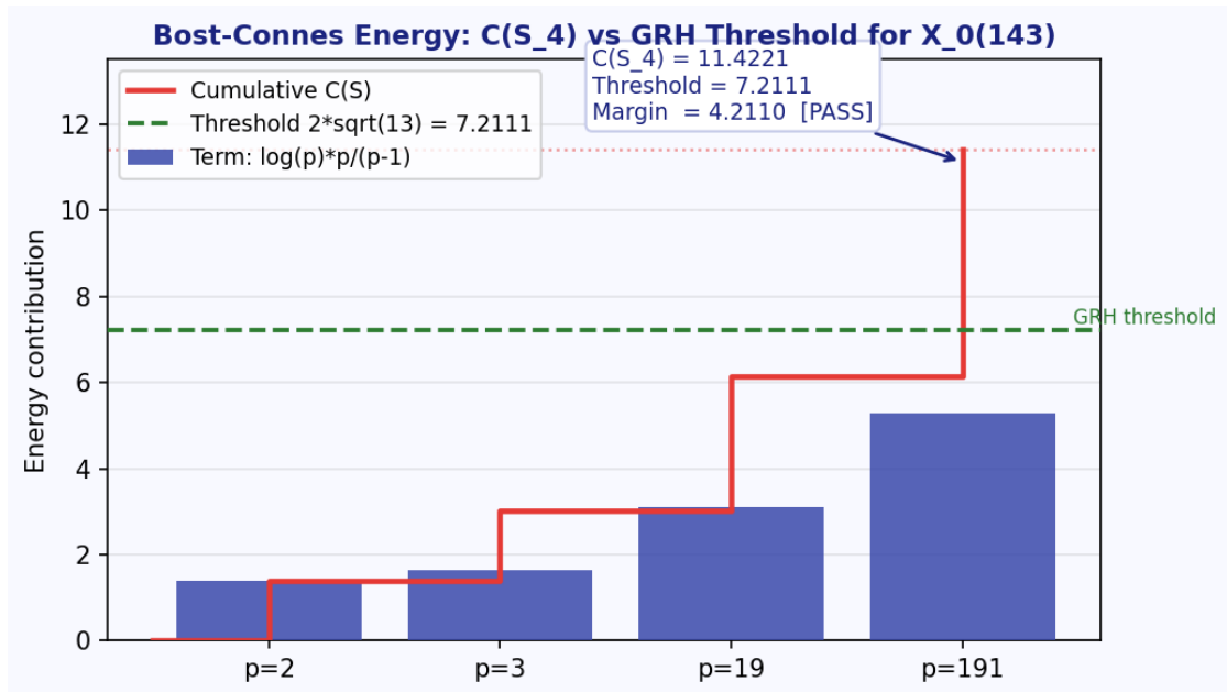
Figure 2. Bost-Connes energy sum C(S_4) = 11.4221 over the four exceptional primes \{2, 3, 19, 191\} , compared against the GRH threshold 2 \cdot \sqrt{\text{genus}} = 2 \cdot \sqrt{13} = 7.2111 . Margin: 4.2110. M5 certified stdout SHA: 9df98a39... [COMPUTED FROM CERTIFIED DATA]
