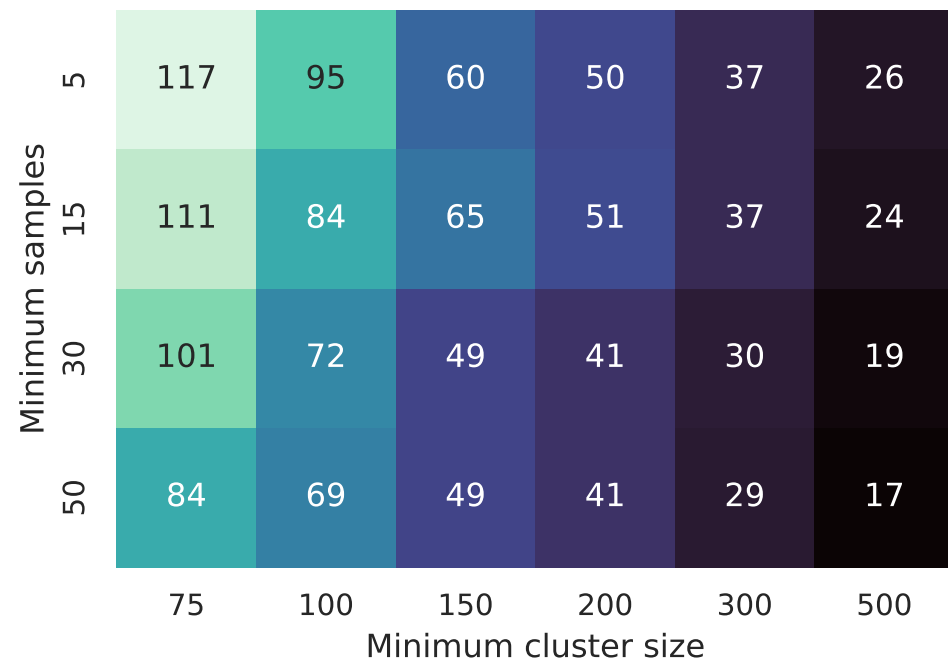
20D • Cluster count
