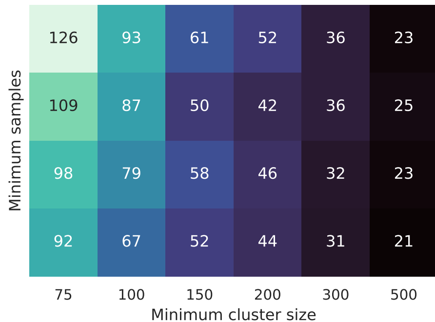
30D • Cluster count
