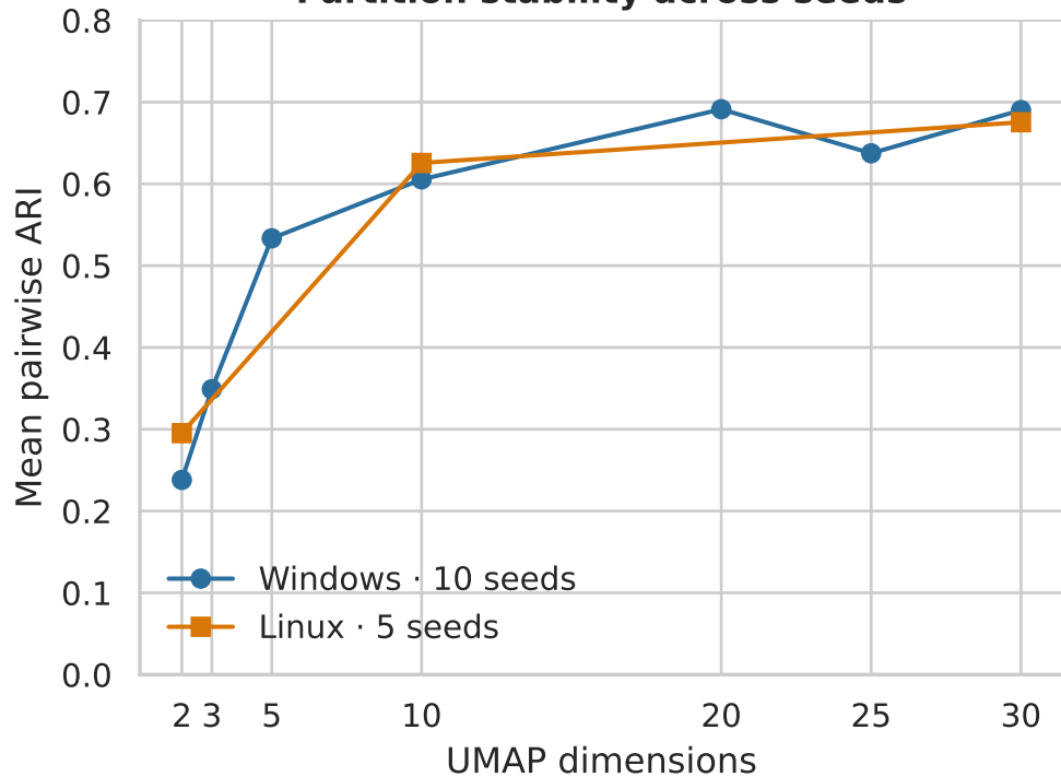
Partition stability across seeds
