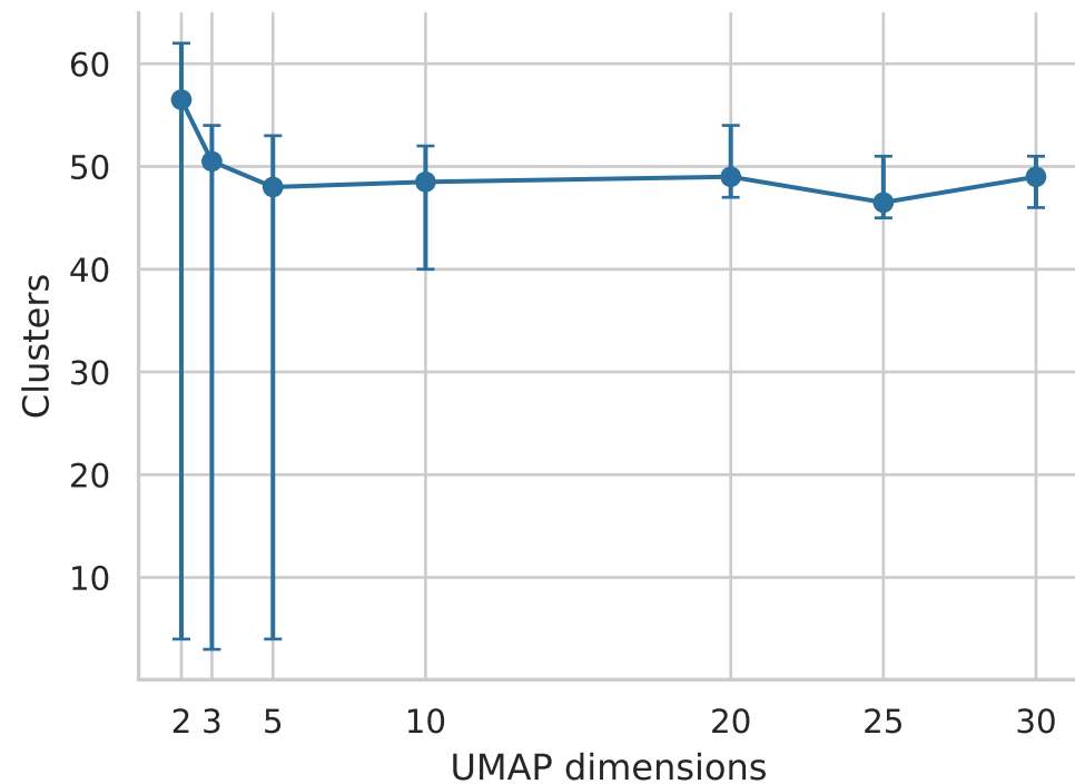
Seed variation in cluster count
