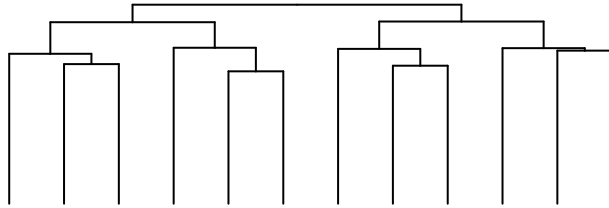
sample correlation matrix genes.count_table.minRow10.CPM.log2.centered
