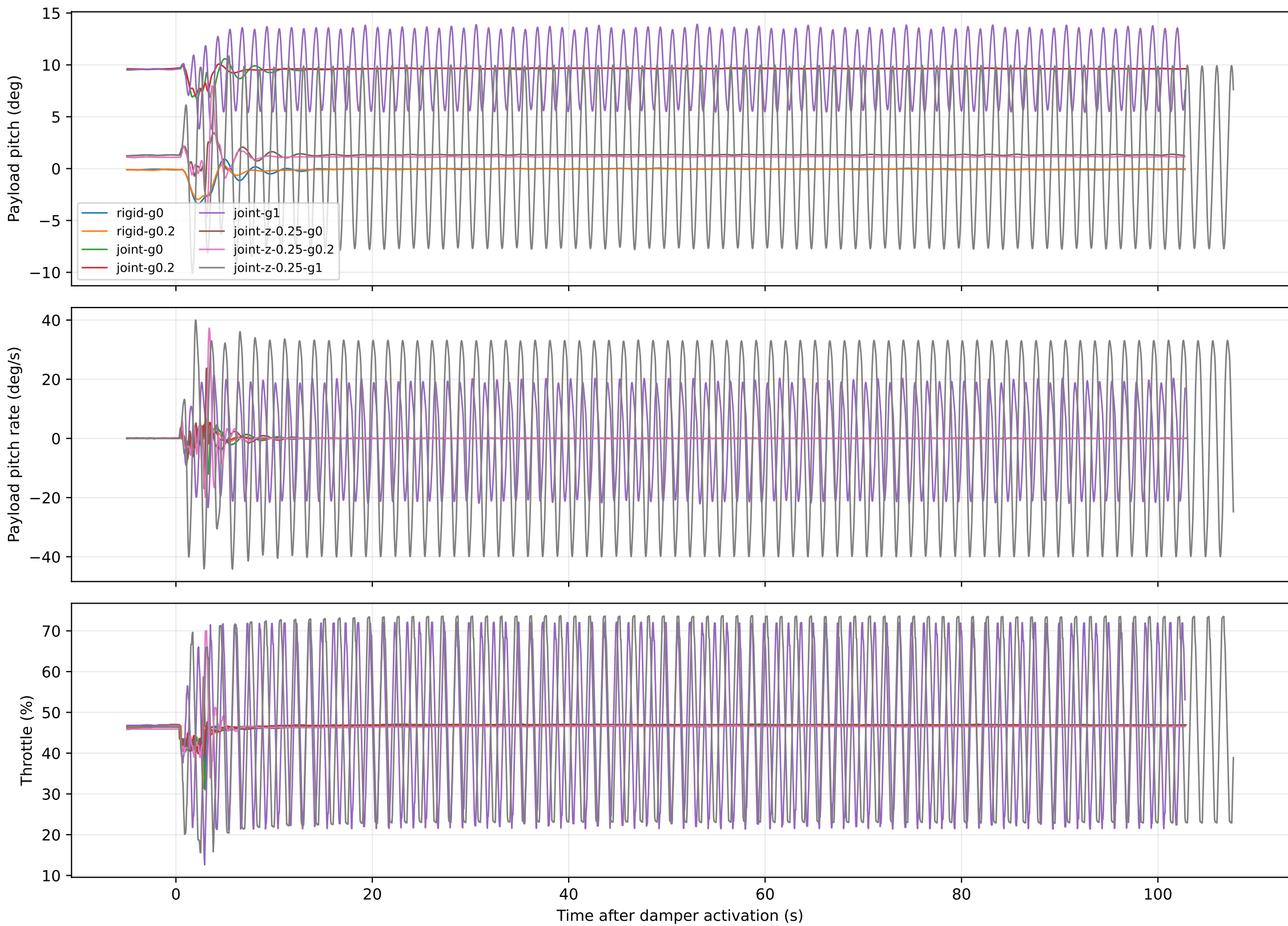
Provisional canopy/payload pitch joint: actual Plane TECS in SITL
