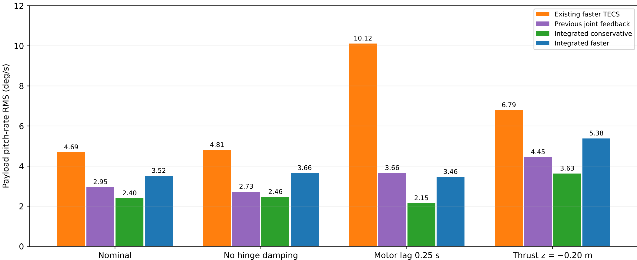
Model sensitivity: actual Plane/SITL, same climb/descent maneuvers Nominal gains retained across each model change; perfect simulated state
