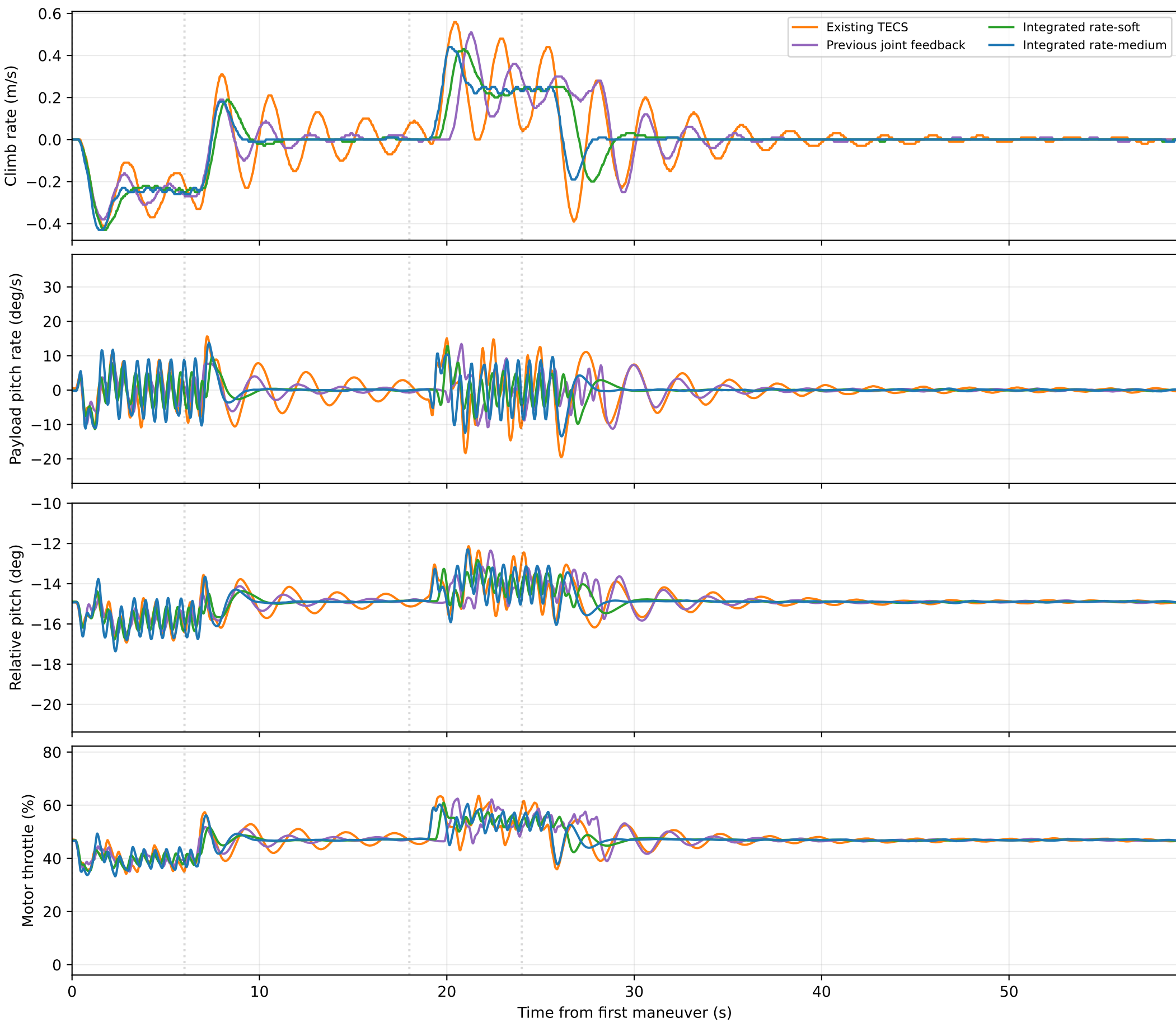
Integrated longitudinal control in actual Plane/SITL Same descent / hold / climb / hold; truth-state benchmark, no observer or stall protection
