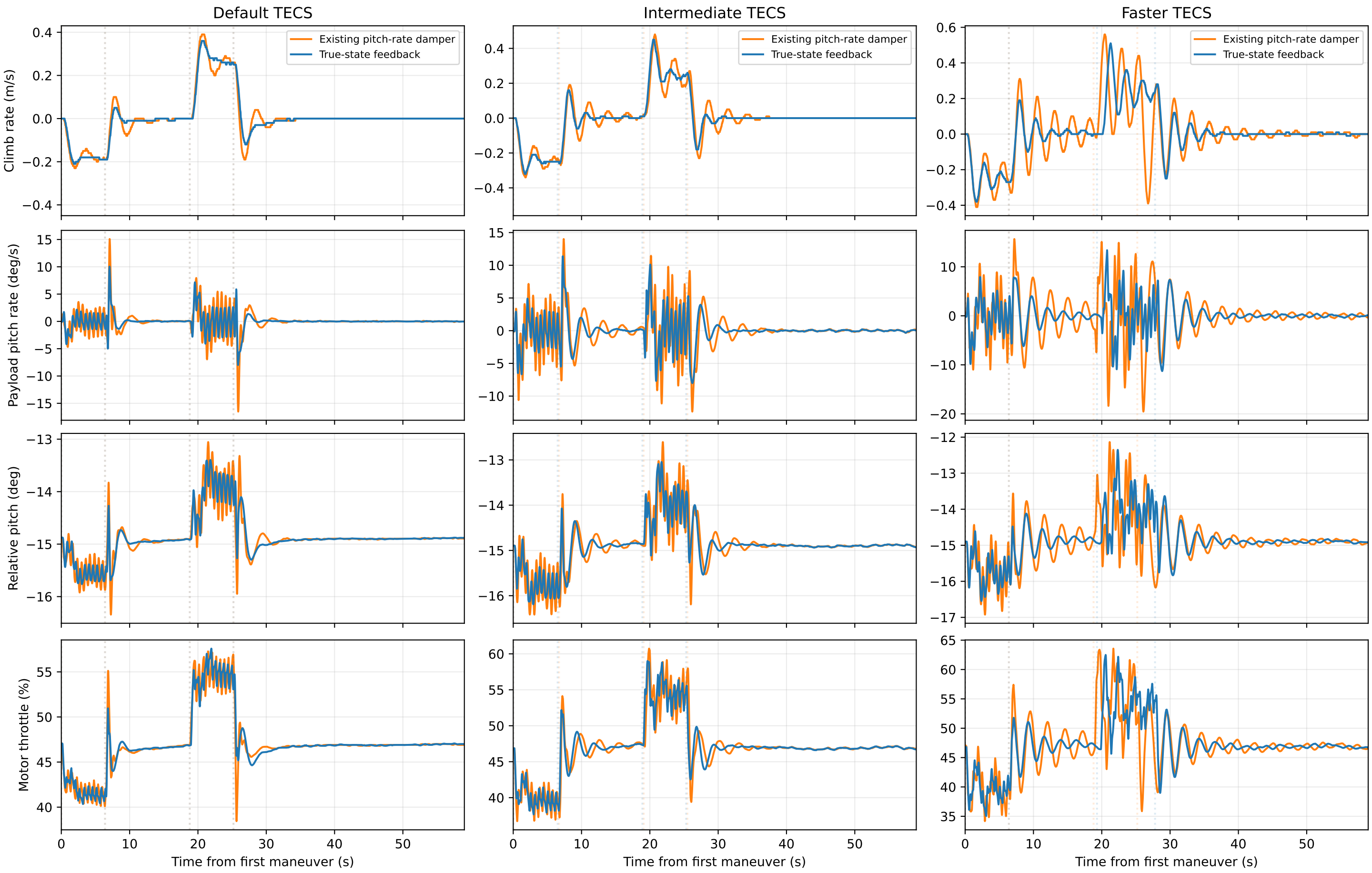
Actual Plane TECS with production flight physics: oracle throttle feedback before motor lag Matched 6 s descent, hold, 6 s climb, hold; airborne preparation; no observer or stall constraint
