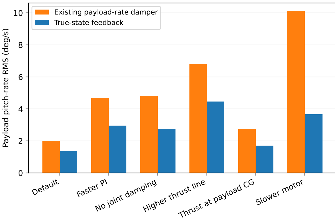
Actual Plane TECS: true relative-rate information adds useful damping Calm matched maneuvers; fixed gains; no stall constraint; motor lag and throttle limits retained
