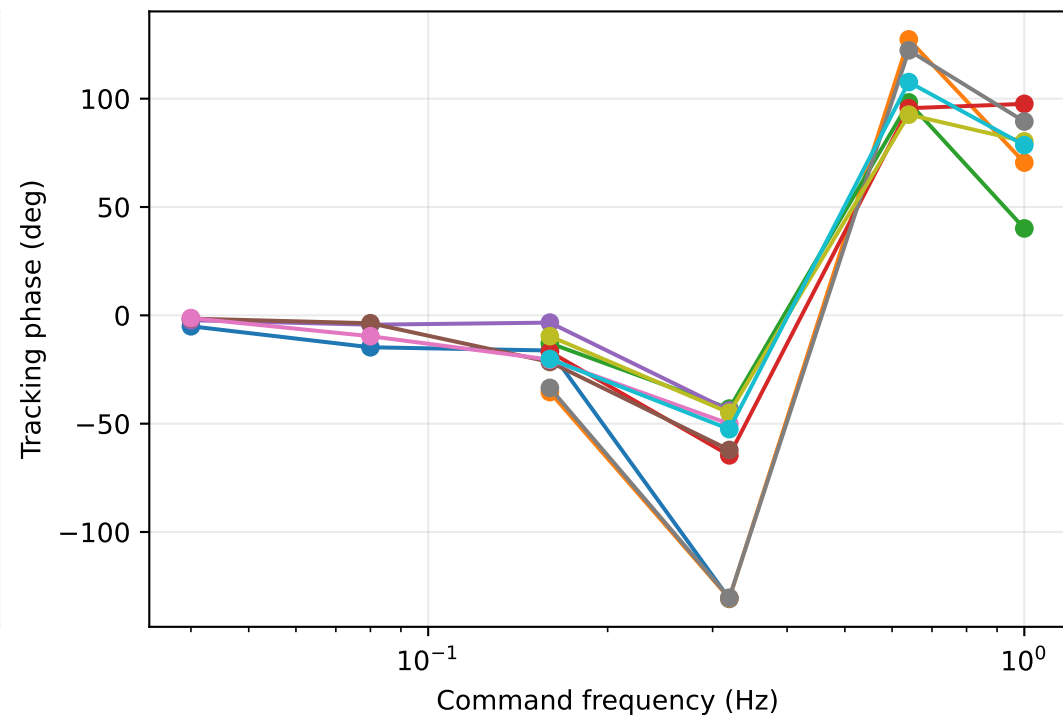
Actual Plane closed-loop frequency response: 0.2 \pm 0.1 m/s climb-rate commands Fit uses logged incoming altitude trajectory and simulated GPS vertical velocity; first cycle excluded
