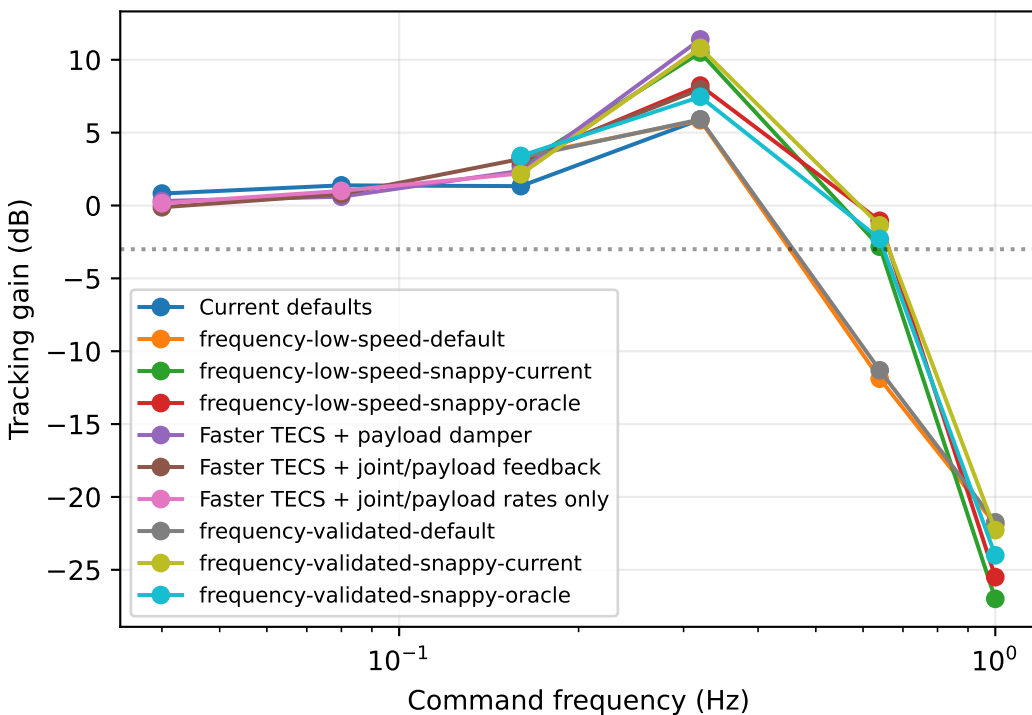
Actual Plane closed-loop frequency response: 0.2 \pm 0.1 m/s climb-rate commands Fit uses logged incoming altitude trajectory and simulated GPS vertical velocity; first cycle excluded
