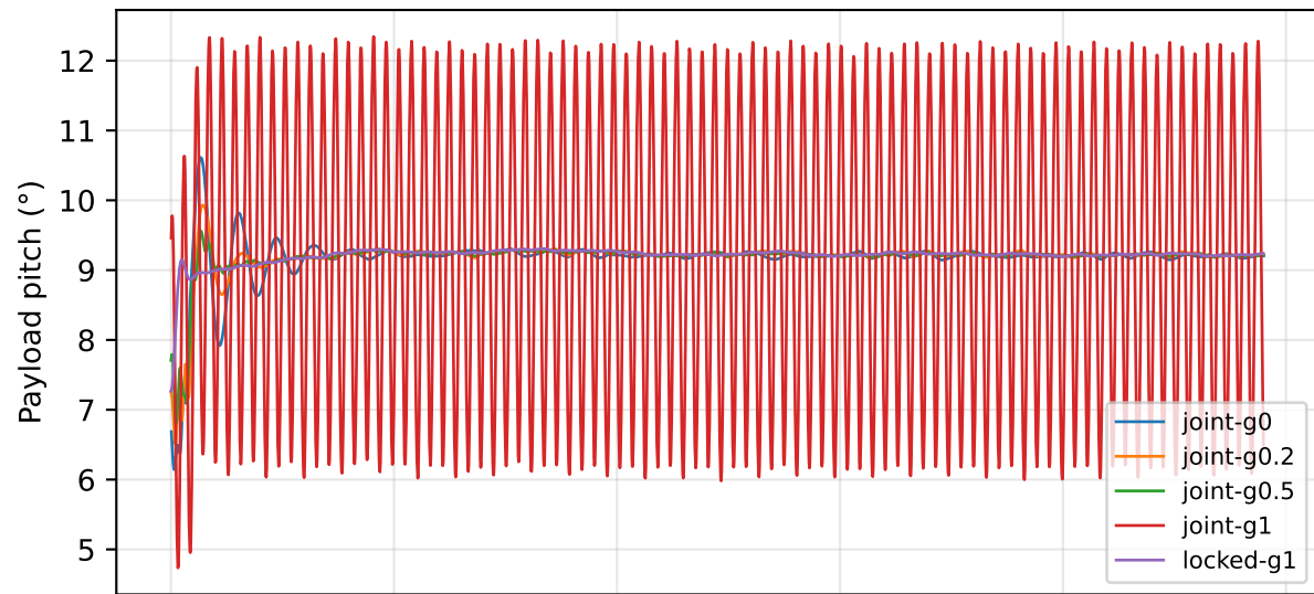
Damper gain and matched locked-joint control
