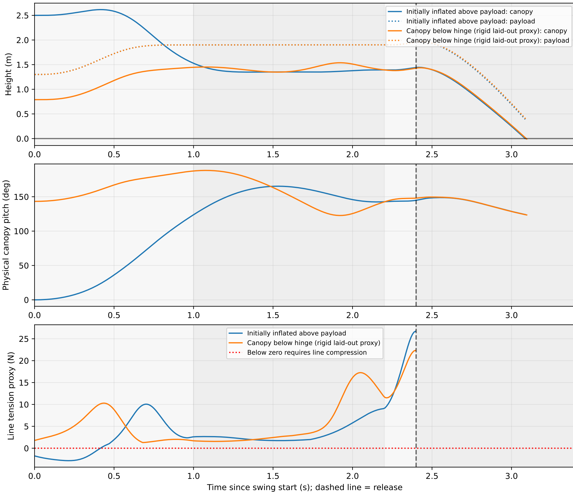
Launch feasibility experiment: inflated rigid-wing physics cannot represent inflation One-second overhead swing, two steps, light toss; throttle remains off for one second after release
