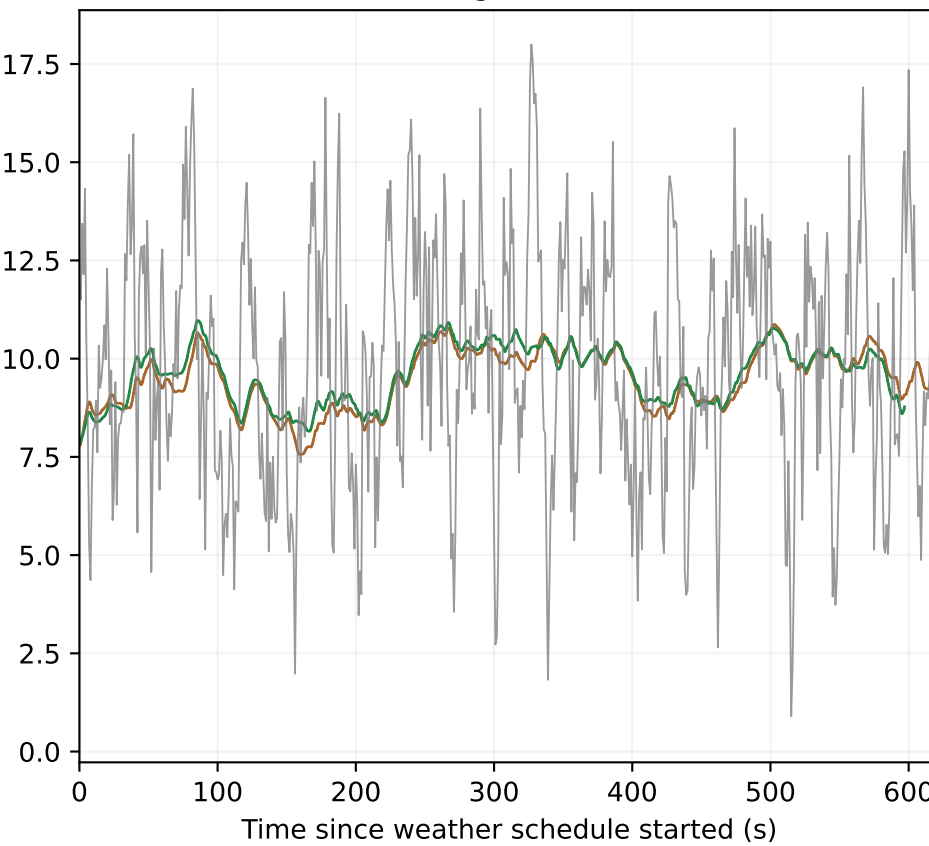
Mean 9.0m/s from 176°; gust \sigma 3.2m/s; turbulence 1.0
