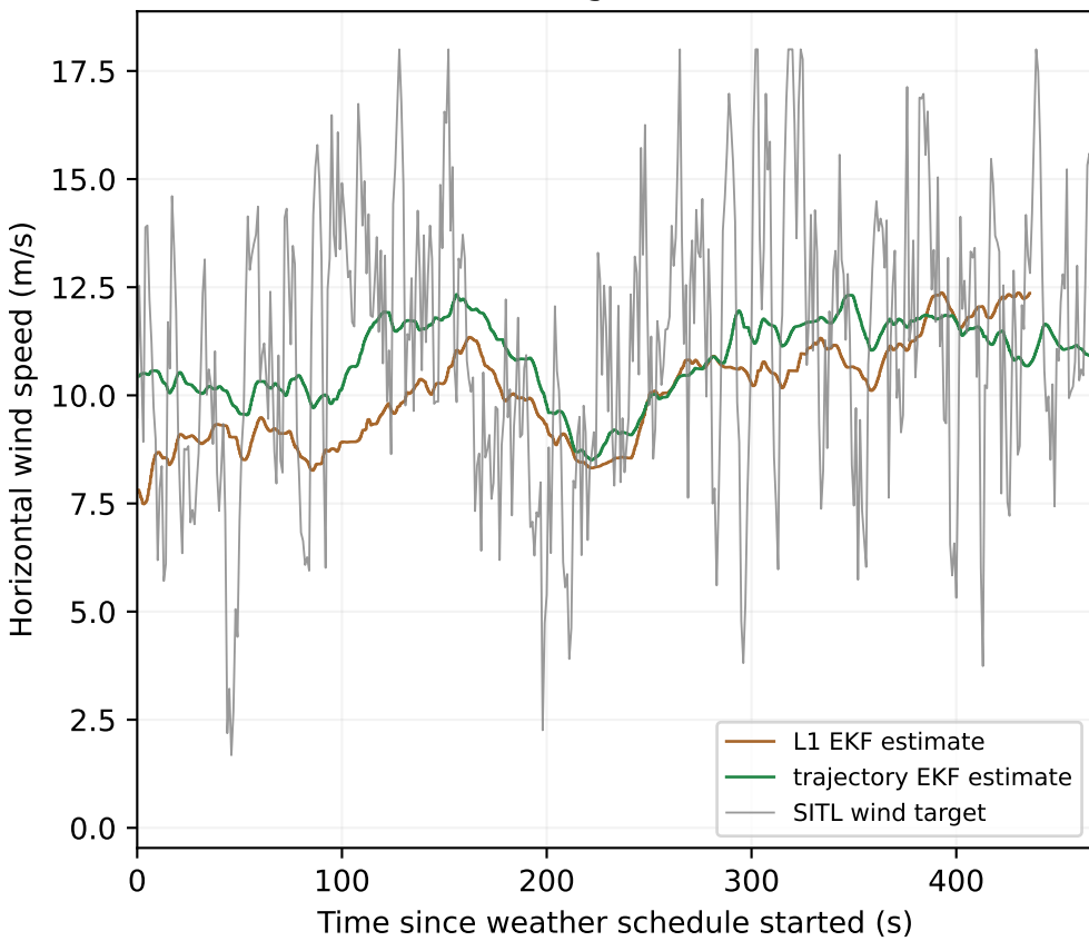
Mean 10.8m/s from 298°; gust \sigma 3.9m/s; turbulence 1.5
