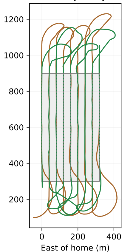
Mean 9.0m/s from 176°; gust \sigma 3.2m/s; turbulence 1.0
