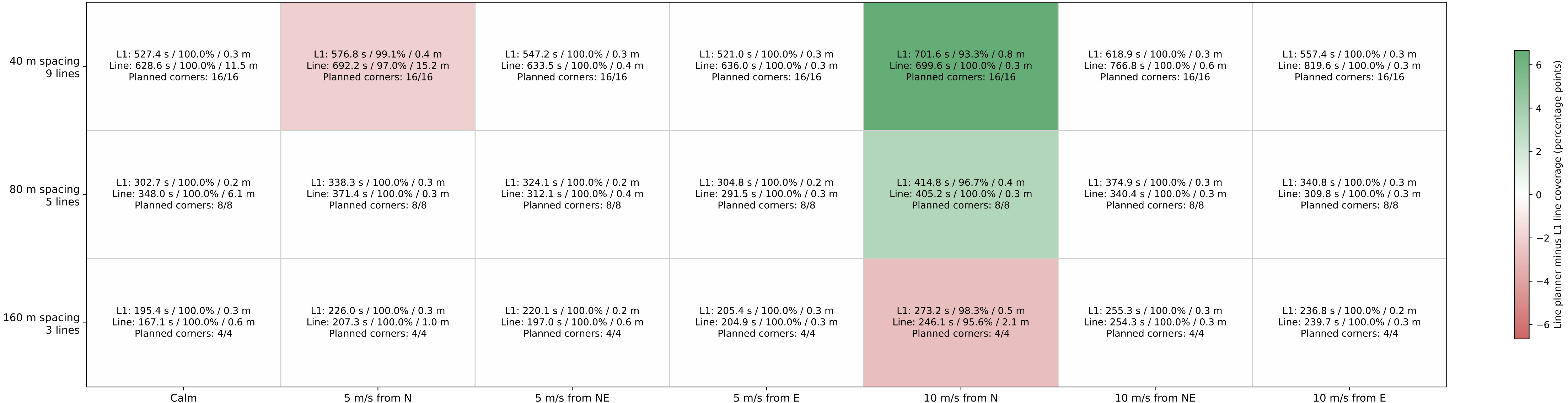
Raster survey matrix: standard L1 versus line-to-line planner Each cell: AUTO course time / requested-line coverage / survey-leg RMS error
