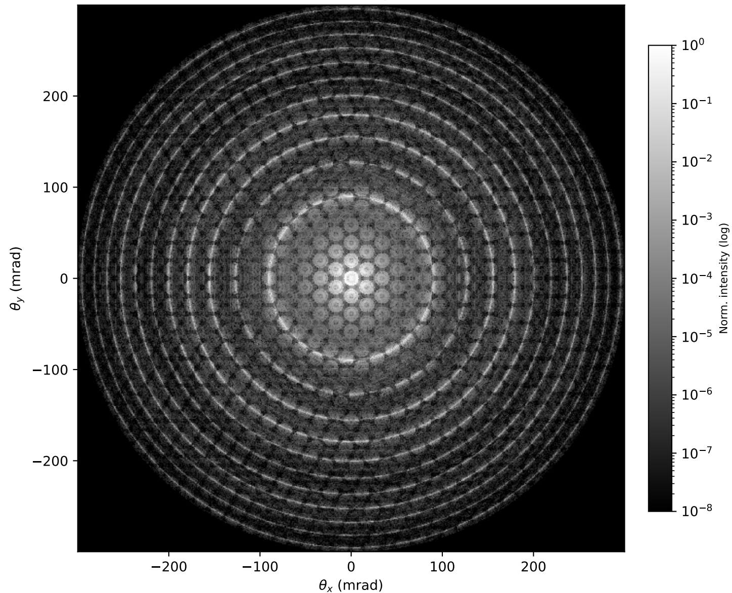
(a) WPM CBED pattern
