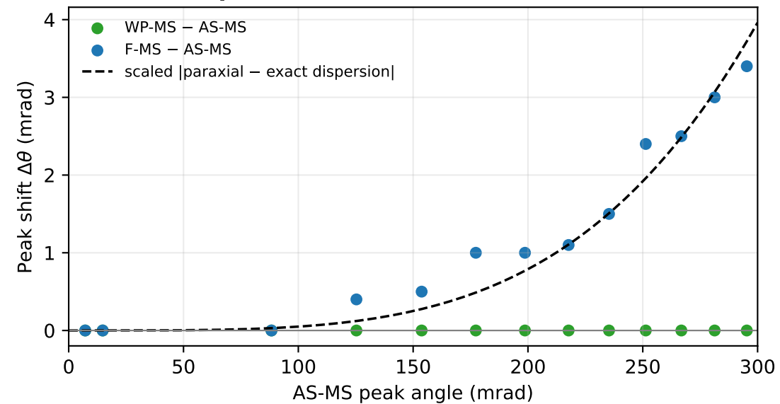
(c) Peak displacement
