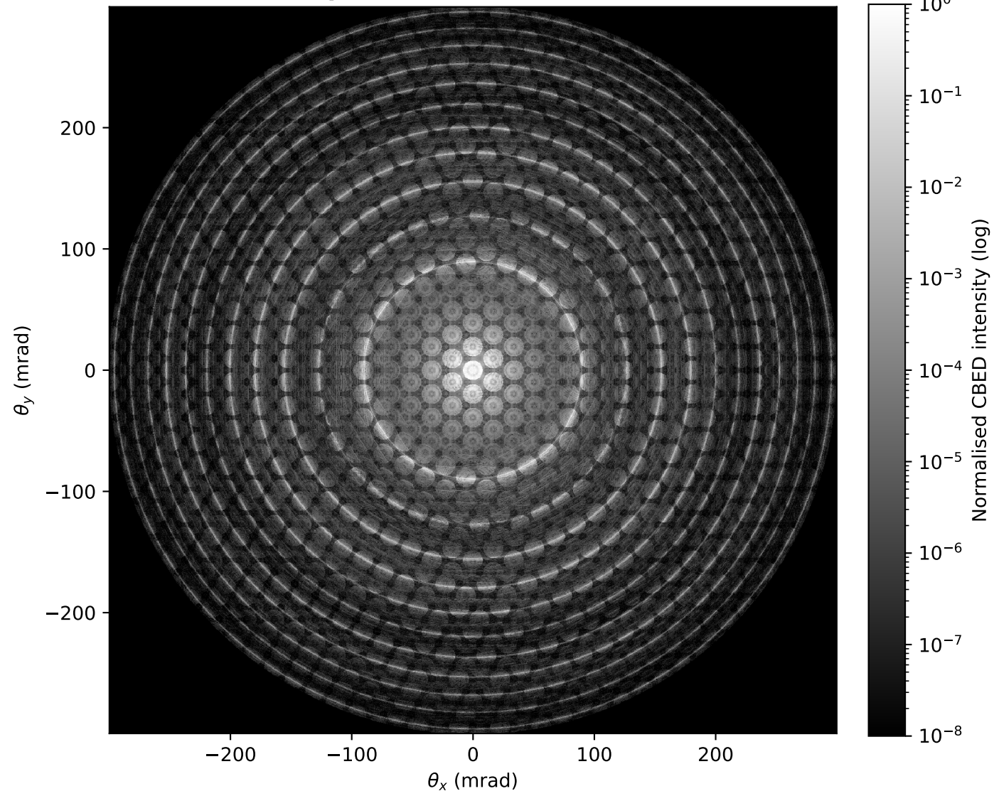
(a) WP-MS CBED pattern
