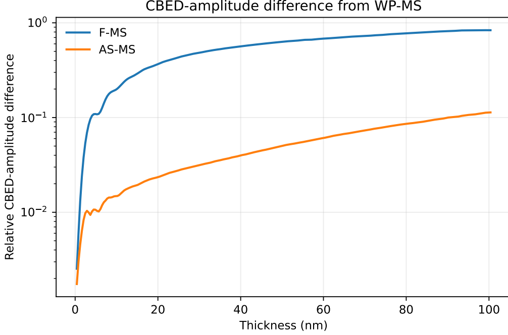
Figure 7: Relative CBED-amplitude differences from the 64-bin WP-MS result as a function of specimen thickness for Au [100] at 200 keV, using a 5 mrad probe and 64 slices per unit cell. Scattering angles up to 300 mrad are included.
