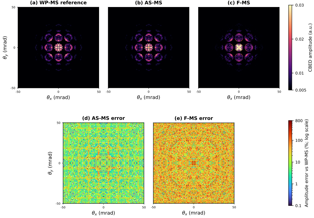
Figure 6: CBED exit-wave amplitude comparison for the Au [100] convergence-angle experiment. The top row shows the final diffraction amplitudes from (a) WP-MS, (b) AS-MS, and (c) F-MS. The lower row shows the pixel-wise amplitude errors of (d) AS-MS and (e) F-MS relative to WP-MS on a logarithmic percentage scale.
