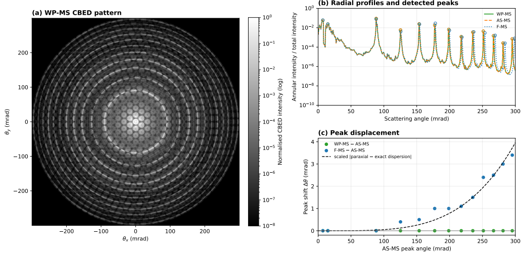
Si [111] CBED — 997.1 Å at 100 keV; 8 mrad probe
