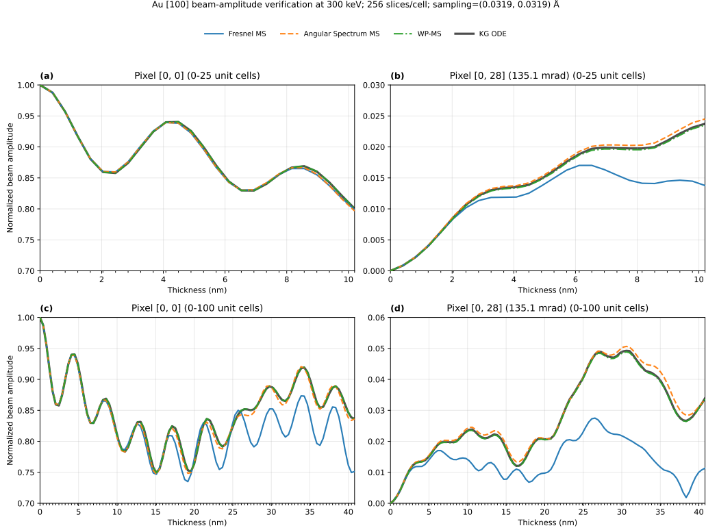
Figure 4: Fourier-component amplitudes for the Au [100] benchmark, with the incident [0, 0] amplitude normalised to unity. Panels (a) and (b) show the first 25 unit cells for the [0, 0] and [0, 28] components, respectively; panels (c) and (d) extend the same comparison to 100 unit cells. The [0, 28] component corresponds to approximately 135.1 mrad.
