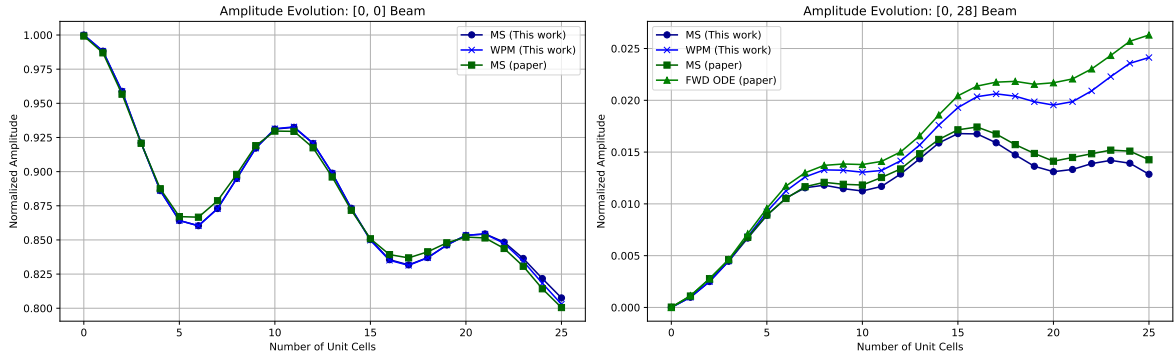
Figure 1: Recreation of figure 3 in [?] showing the amplitude of the central and high angle (135 mrad) diffracted beams, after propagation with our multislice and wave propagation methods. Plotted in green is the "ground truth" ODE solution, and the multi-slice solution of to the Klein-Gordon equation. In blue is the Angular Spectrum Multislice (ASMS) solution and the Wave Propagation Method (WPM) solution
