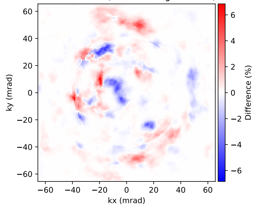
Diffraction Diff (WPM binning - Fresnel)
