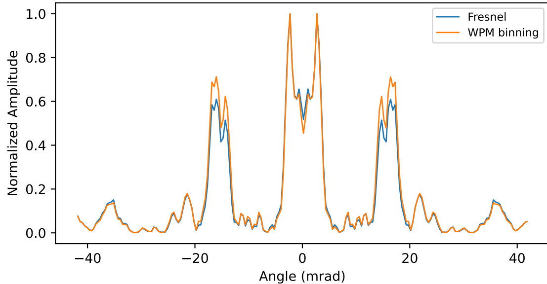
Diffraction center-row cross-section
