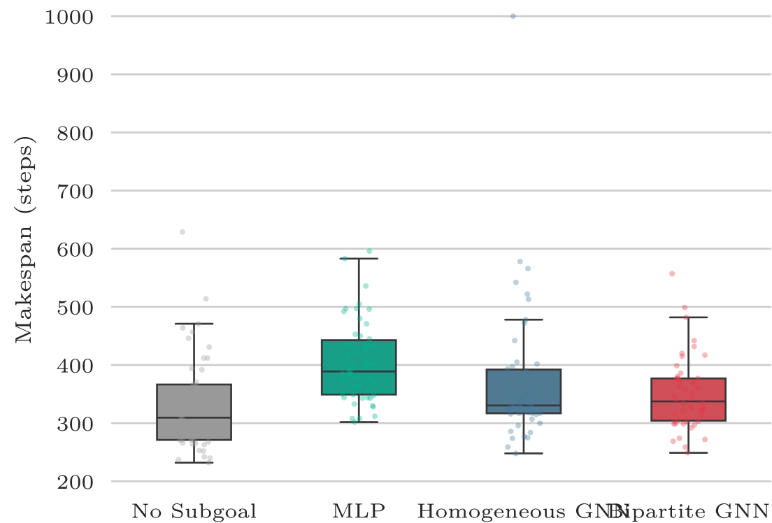
Makespan Distribution
