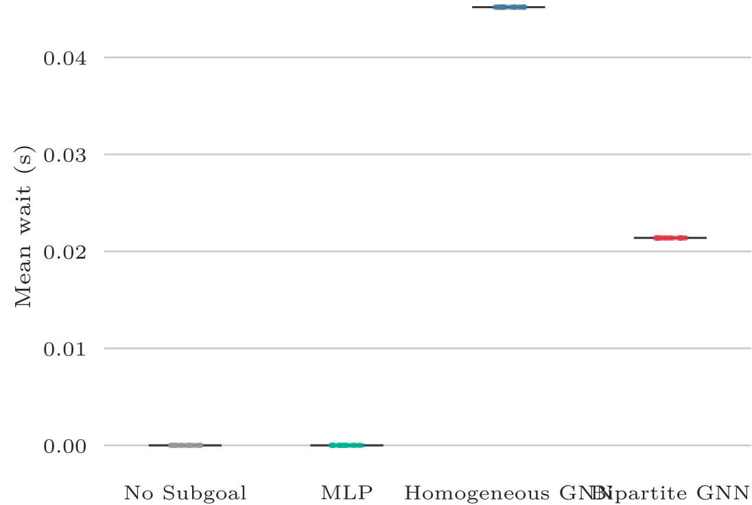
Mean Prescribed Wait Time (0 = no subgoal)
