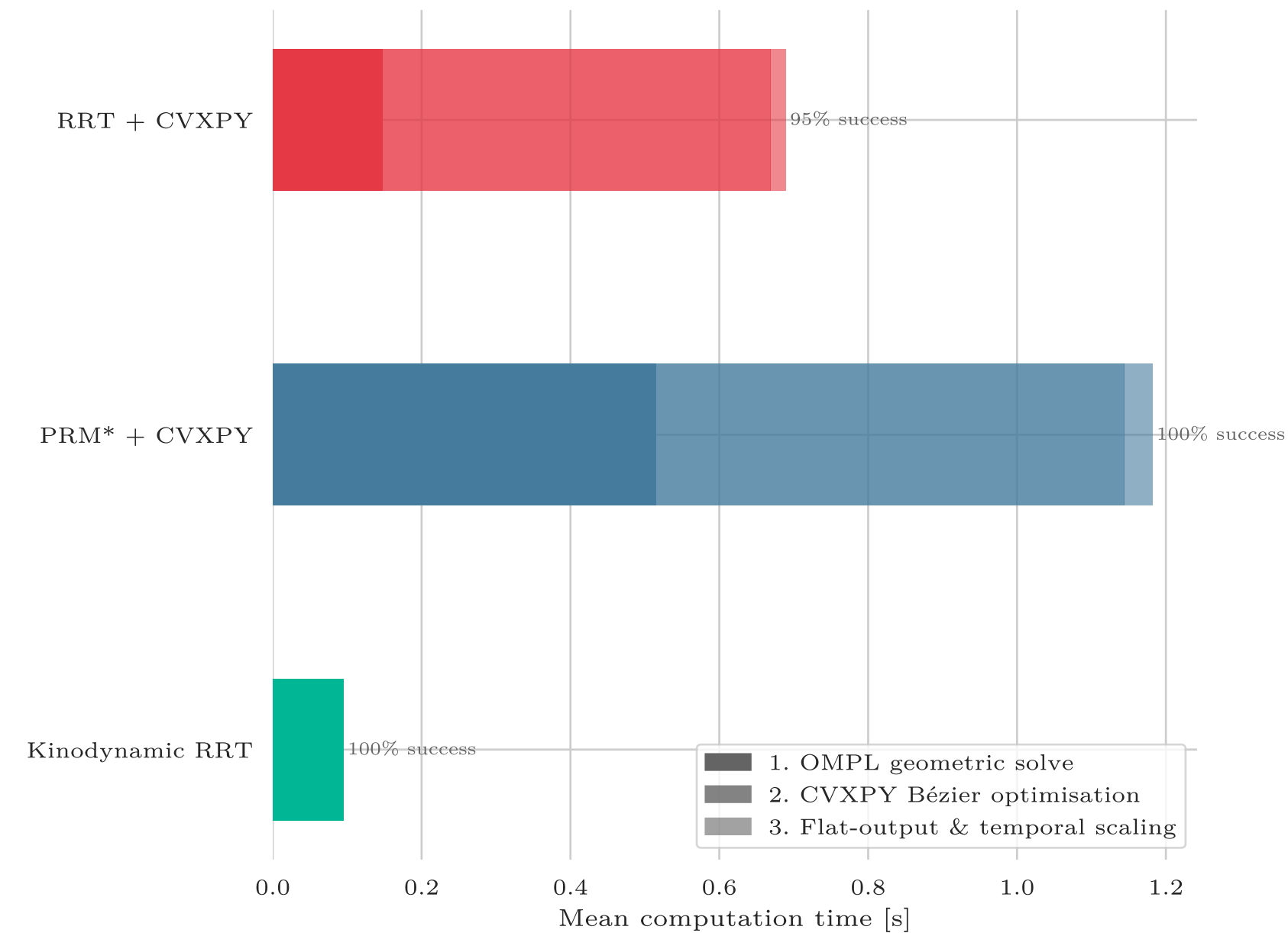
Motion Planning Pipeline Timing
