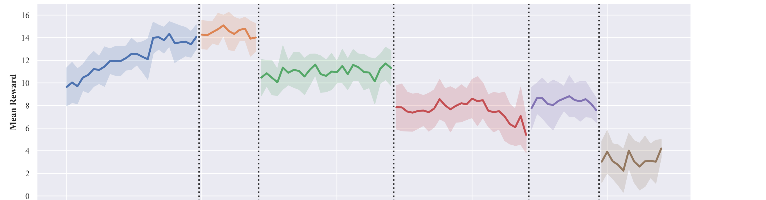
Training Progress: Reward
